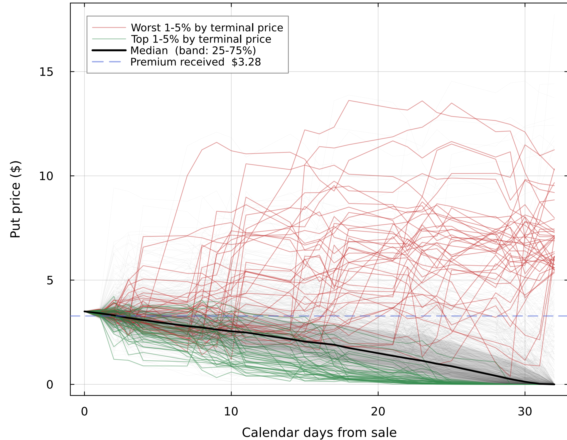
Short 32-calendar-day 30 \Delta put: option price
