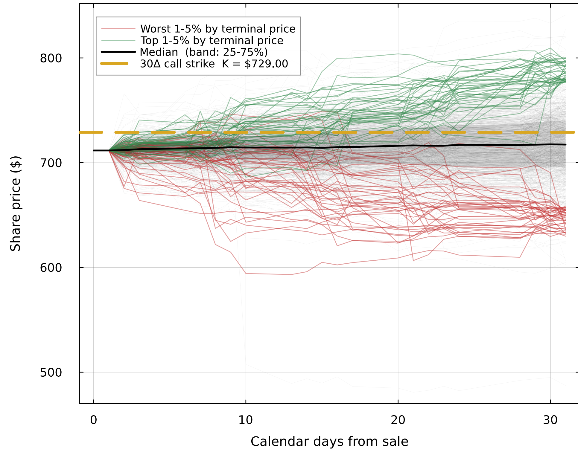
SPY share price paths ( S_0 = \$711.68 )
