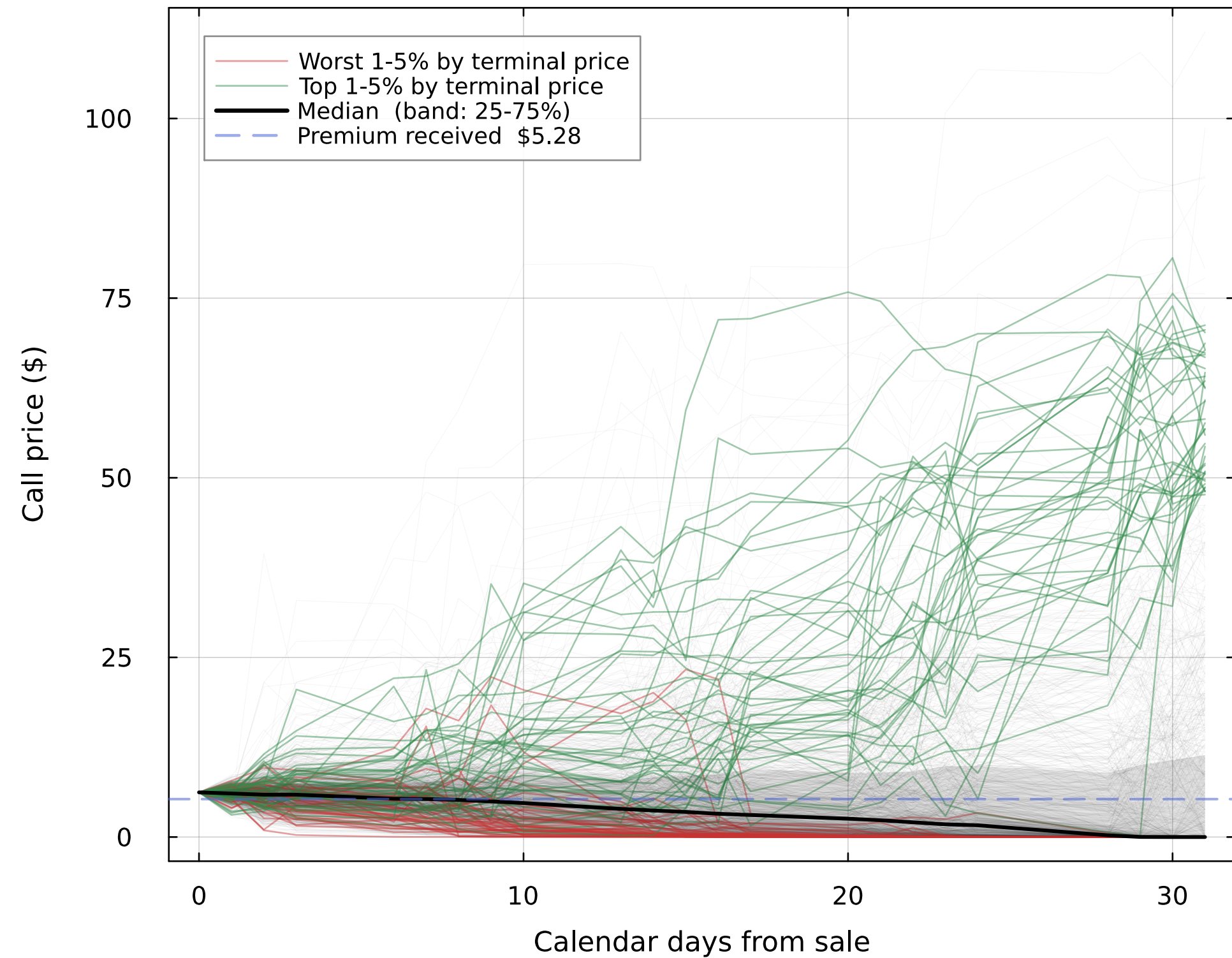
Short 31-calendar-day 30 \Delta call: option price
