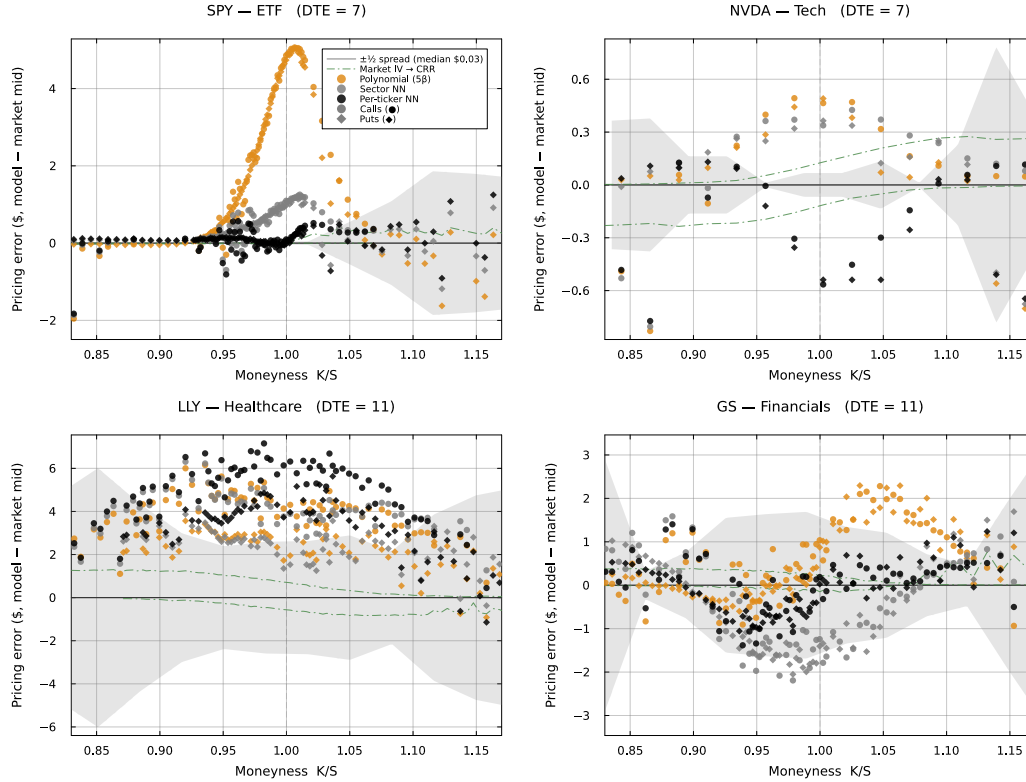
Figure 2: In-sample comparison of CRR American-option prices with Alpaca indicative mids across moneyiness for SPY, NVDA, LLY, and GS on May 11, 2026. Errors are tree price minus indicative mid. Curves show prices from the parametric, sector, and per-ticker surfaces and, for reference, from the reported IV. The gray ribbon is the median local bid-ask half-spread by moneyiness bin. A point inside the ribbon has an absolute pricing error below that local half-spread.
