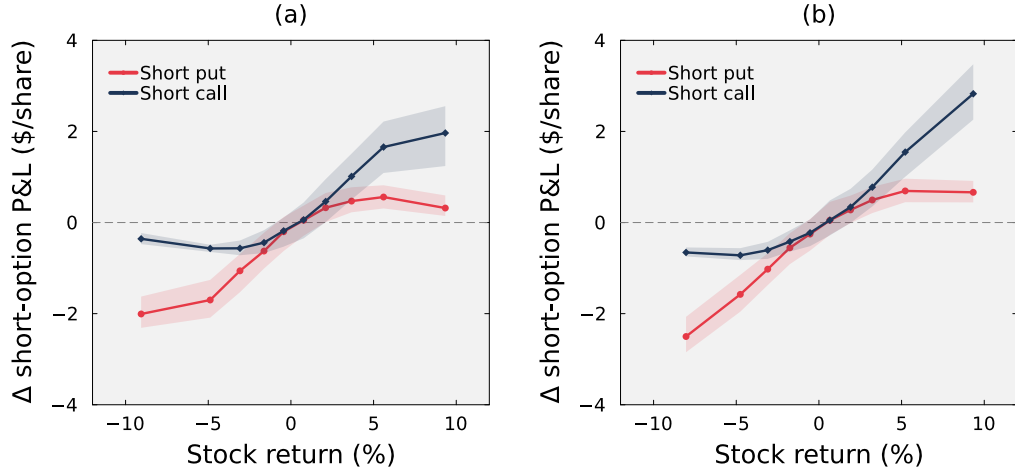
Figure 5: Effect of linking IV shocks to stock returns on short-option P&L before expiration, by stock return, after ten trading days for (a) GS and (b) LLY. Each difference is full-factor P&L ( \rho = -0.6 ) minus uncoupled-factor P&L ( \rho = 0 ) on the same stock path, with the same independent normal shocks. Negative values indicate worse short-position P&L under coupling. The 3,000 paths per ticker are sorted by stock return and divided into ten groups of 300. Symbols show each group’s median P&L difference at its median stock return, and lines connect the symbols. Shaded bands span each group’s 25th–75th percentiles. These bands describe variation across paths, not confidence intervals. Red circles denote puts and navy diamonds denote calls. All prices are evaluated on May 12, 2026, with 17 calendar days to expiration.
