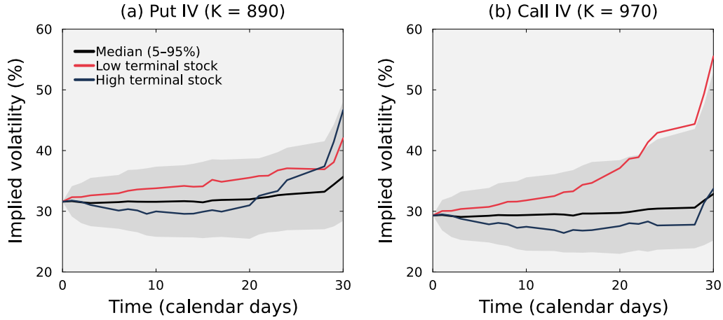
Figure 4: Simulated evolution of annualized IV at the GS put strike (a) and call strike (b) in the scenario of Fig. 3. Both panels express IV as percentages on the same vertical scale. Curves show pointwise medians across all 1,000 paths and within the terminal-stock groups defined in Fig. 3. Shading shows the 5th–95th percentile band. Time is measured in calendar days from April 28, 2026, and stops before expiration because the payoff at expiration does not depend on IV.
