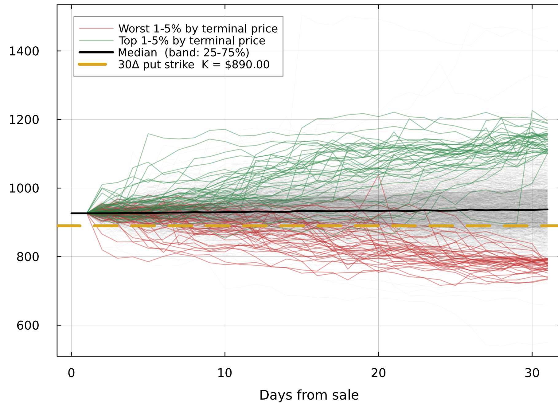
GS share price paths ( S_0 = \$926.38 )
