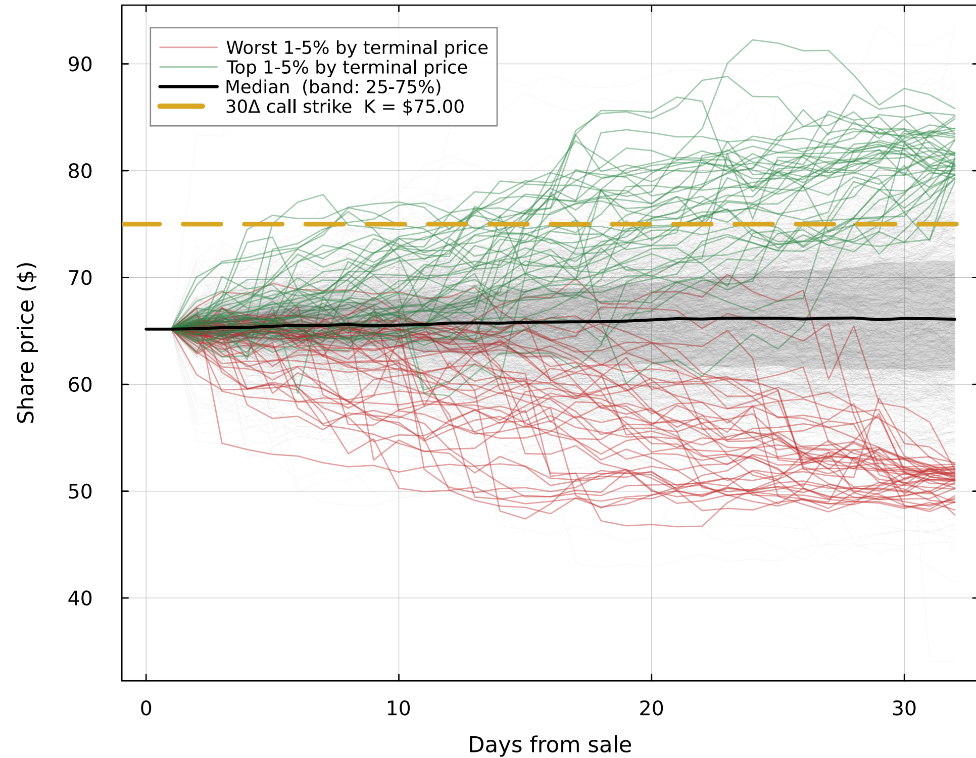
INTC share price paths ( S_0 = \$65.17 )
