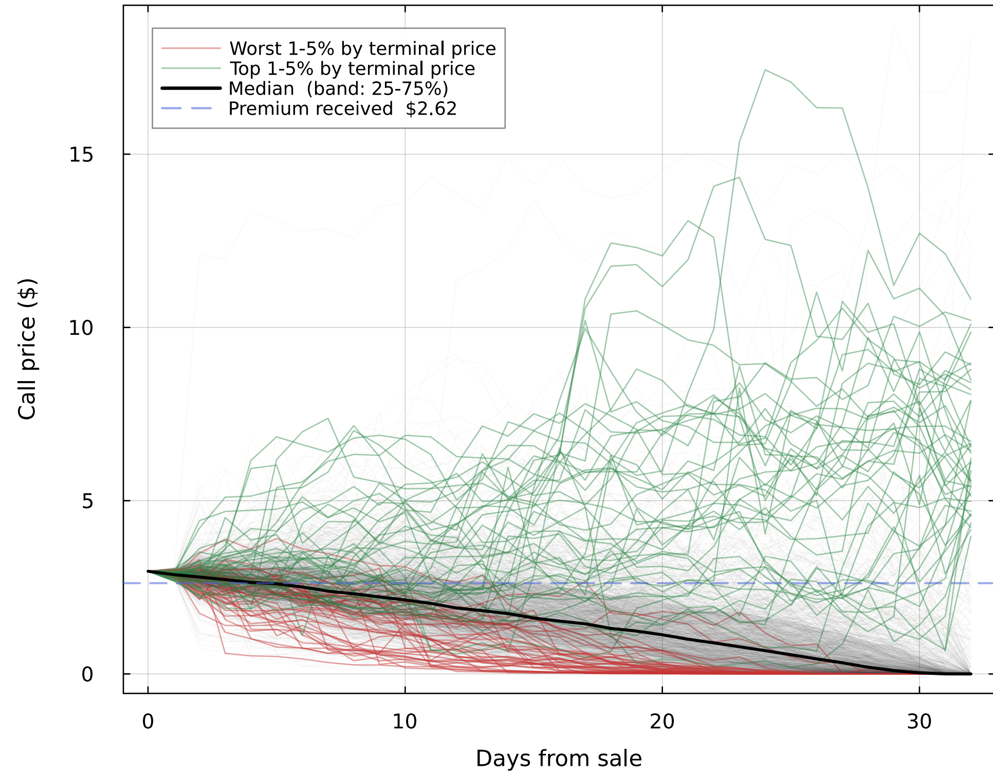
Short 30-day 30Δ call — option price
