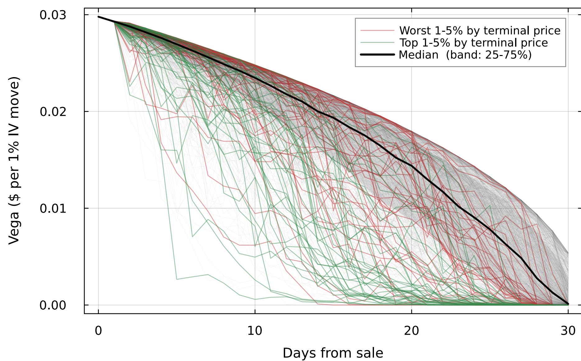
Vega at K_put
