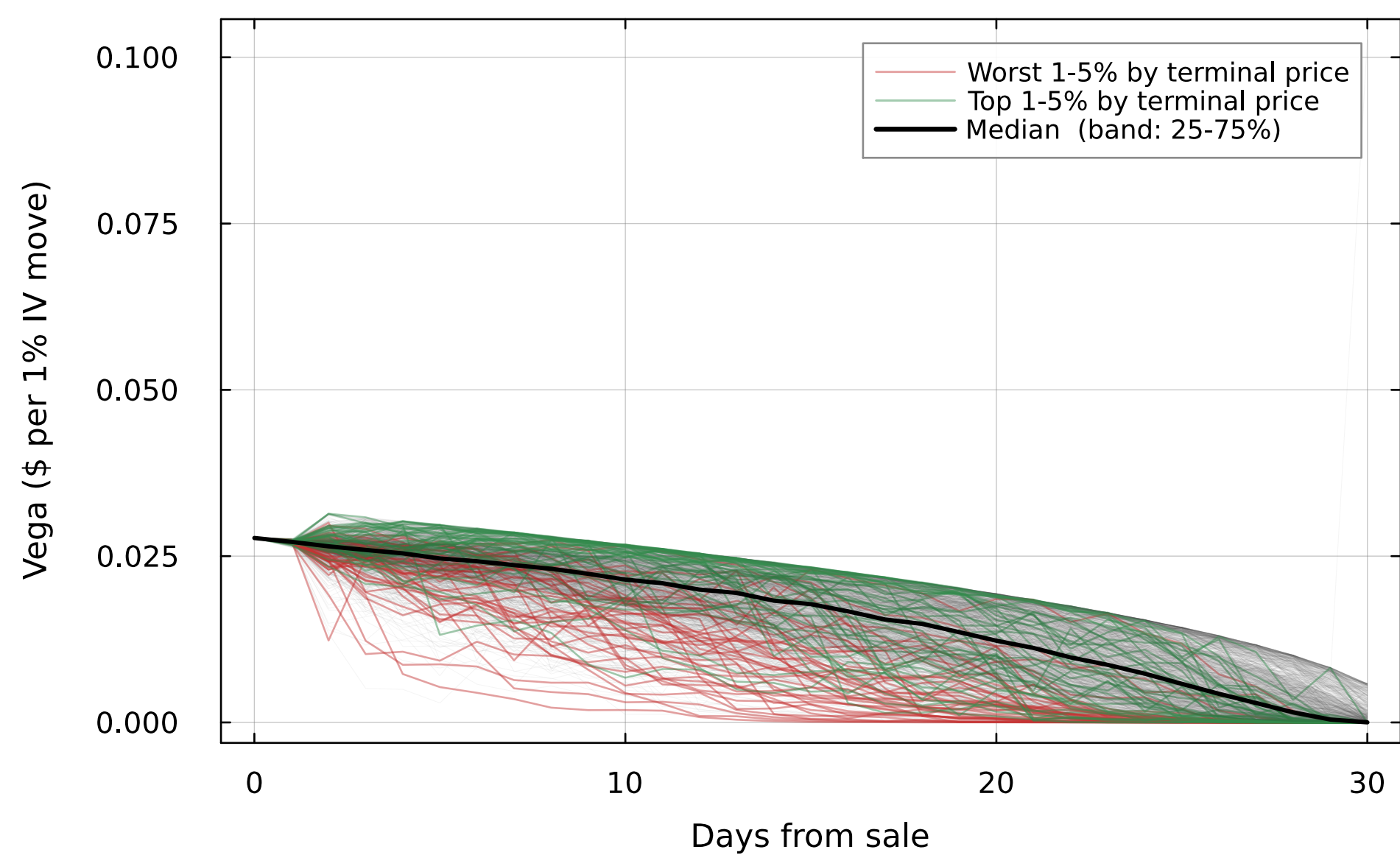
Vega at K_call
