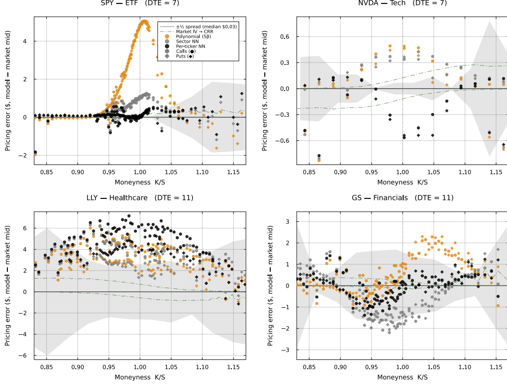
Figure 2: Model-vs-market dollar pricing error (CRR American at the calibrated IV minus market mid) versus moneyiness for SPY (DTE 7), NVDA (DTE 7), LLY (DTE 11), and GS (DTE 11) on the 2026-05-11 capture. Four model tiers are overlaid on each panel: parametric \psi (light), sector \psi_{NN} (medium), per-ticker \psi_{NN} (dark), and market-IV reference (green dot-dash; yfinance IV repriced through CRR, near zero by construction). The gray ribbon was the local \pm \frac{1}{2} bid-ask spread band, computed per panel by partitioning the contracts into twelve equal-width moneyiness bins, taking the median half-spread (ask — bid)/2 within each bin, and linearly interpolating the twelve bin values onto a fine moneyiness grid. A point falling inside the band was a model error smaller than the typical bid-ask spread at that moneyiness, i.e., a price within the range the market itself was quoting; the band widened toward the wings because bid-ask spreads were systematically larger for deep in- and out-of-the-money contracts. The per-ticker fit dominated parametric and sector tiers on SPY and GS, matched them on NVDA, and showed a uniform positive bias on LLY consistent with the per-ticker \psi encoding the time-averaged IV across fifteen capture dates and the sampled day (05-11) being calmer than the calibration-window average.
