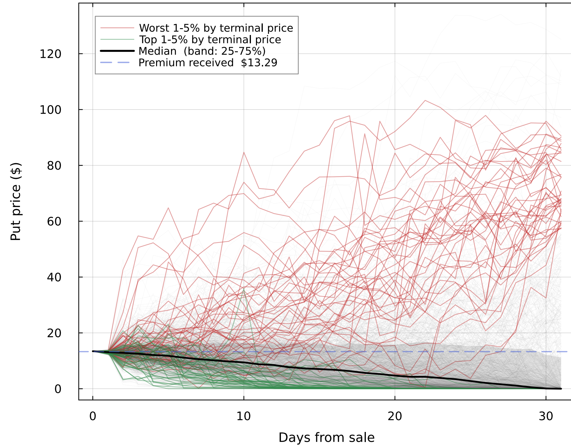
Short 30-day 30Δ put — option price
