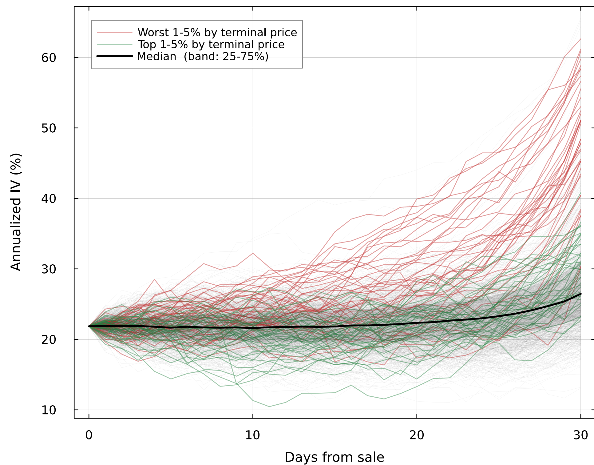
Implied volatility at the call strike (K = $235.0)
