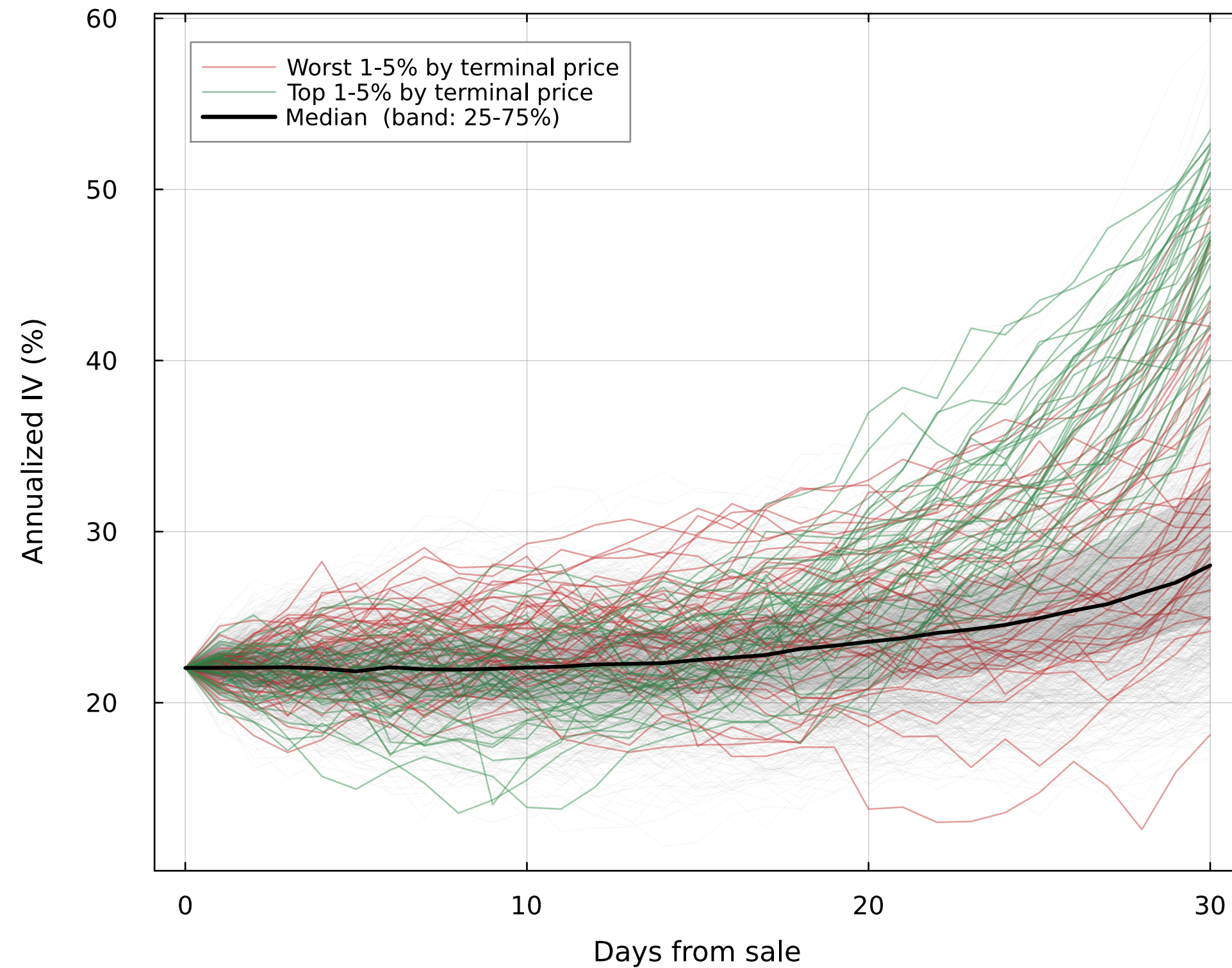
Implied volatility at the put strike (K = $220.0)
