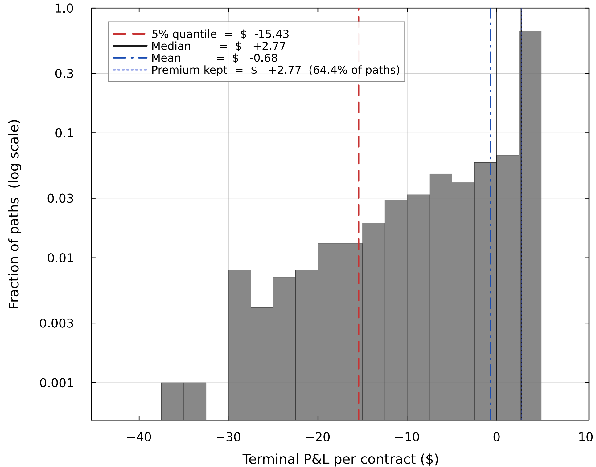
Short 30-day 30 \Delta call — terminal P&L distribution
