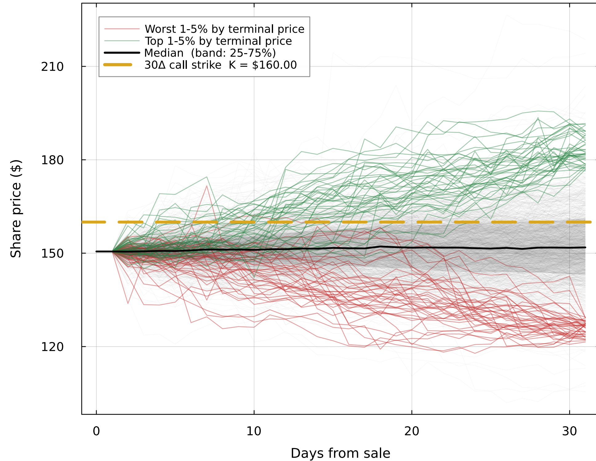
XOM share price paths ( S_0 = \$150.55 )
