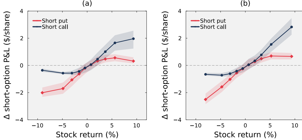
Figure 5: Change in simulated short-option P&L at the fixed horizon of ten trading days caused by linking IV shocks to stock returns, for (a) GS and (b) LLY. Each difference is full-factor P&L ( \rho = -0.6 ) minus uncoupled-factor P&L ( \rho = 0 ) on the same stock path, with the same independent normal shocks. Negative values indicate worse short-position P&L under coupling. The horizontal axis is each path's stock return from entry on April 28 to May 12. The 3,000 paths per ticker are sorted by this return and divided into ten groups of 300. Symbols show each group's median P&L difference at its median stock return, and lines connect the symbols. Shaded bands span each group's 25th–75th percentiles. These bands describe variation across paths, not confidence intervals. Red diamonds denote puts and navy circles denote calls, as in Figs. 1 and 2. All prices are evaluated on May 12, 2026, with 17 calendar days to expiration.
