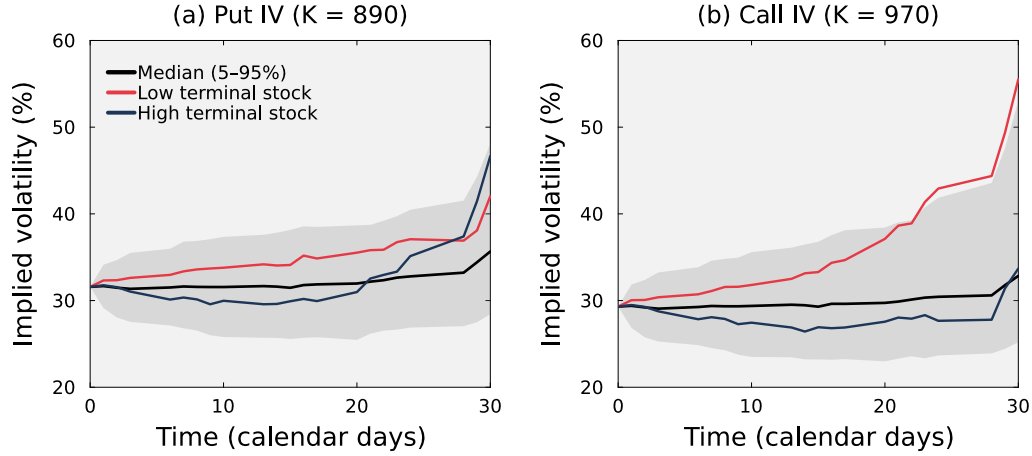
Figure 4: Simulated evolution of the annualized IV of the GS put (a) and call (b) in the scenario of Fig. 3. Both panels express IV as percentages on the same vertical scale. Curves show pointwise medians across all 1,000 paths and within the terminal-stock groups defined in Fig. 3. Shading shows the 5th–95th percentile band across all 1,000 paths. Time is measured in calendar days from April 28, 2026, and stops before expiration because the payoff at expiration does not depend on IV.
