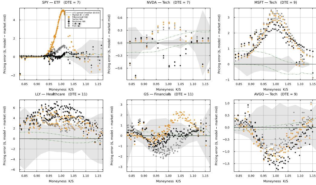
Figure 2: In-sample comparison of CRR American-option prices with Alpaca indicative mids across moneyiness for SPY, NVDA, MSFT, LLY, GS, and AVGO on May 11, 2026, at the maturities of Fig. 1. Errors are tree price minus indicative mid. Points show errors of prices from the parametric, sector, and per-ticker surfaces, with circles for calls and diamonds for puts. Dash-dotted curves show, for reference, errors of prices from each contract’s reported IV. The gray ribbon spans plus and minus the median bid–ask half-spread in each moneyiness bin. A point inside the ribbon has an absolute pricing error below the typical half-spread at that moneyiness. The shares reported in the text instead compare each contract with its own half-spread.
