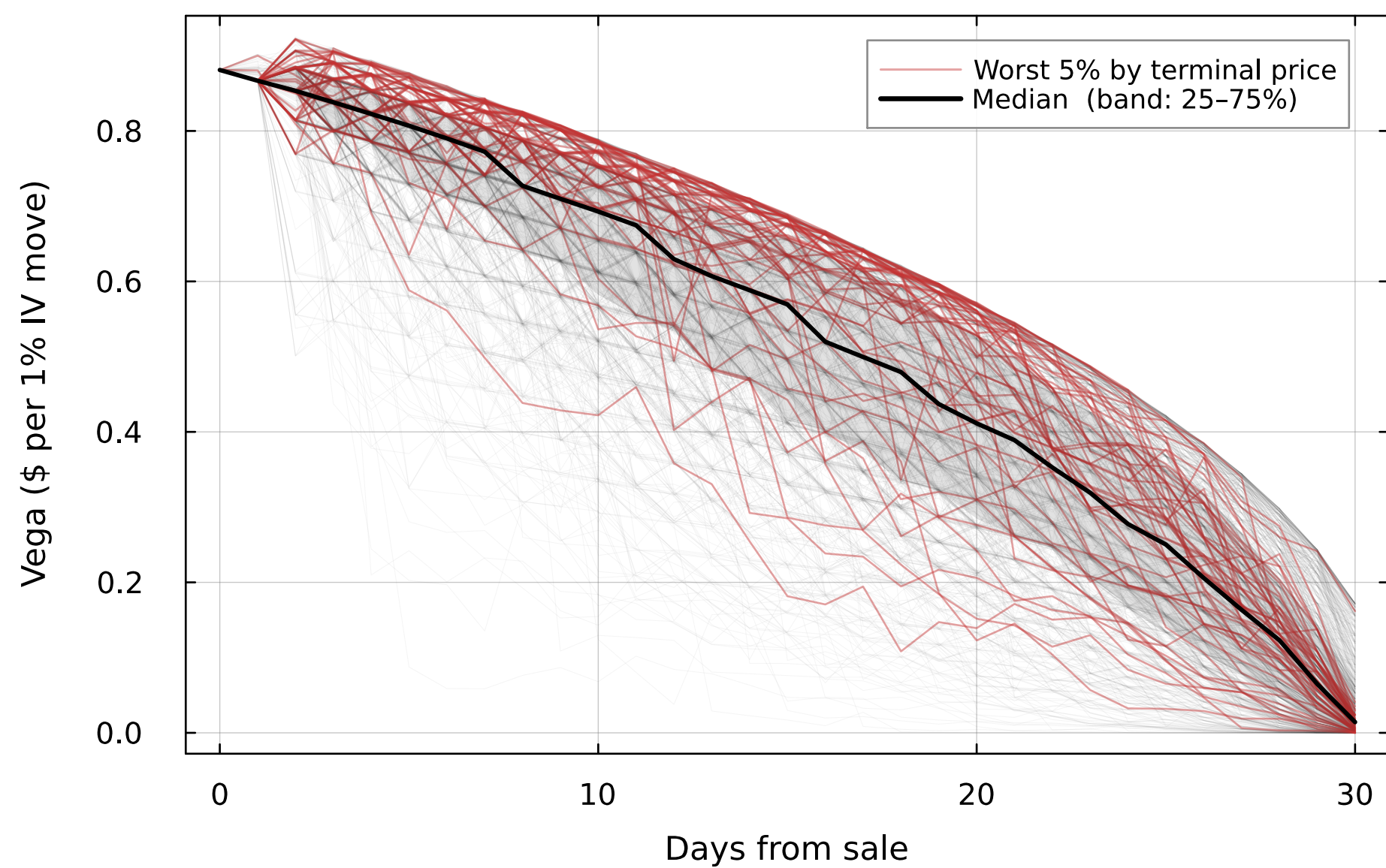
Vega at K_{\text{put}}
