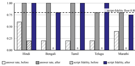
Fig. 4. Per-language acceptance, before and after the two repairs. Answer rate and script fidelity failed for different reasons and were repaired by different changes; the dashed line is the script-fidelity floor, which Marathi does not clear.
