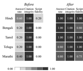
Fig. 5. The three gate measures across both panels. Citation integrity is uniformly 1.00 in each: the structural guarantee held while the tuned behaviour around it was wrong.
