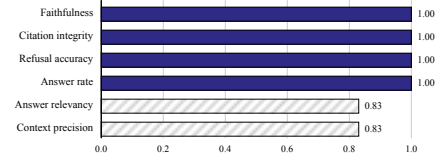
Fig. 6. Reference-free scores. Solid bars are quantities the design guarantees structurally; hatched bars are measured but not guaranteed.
