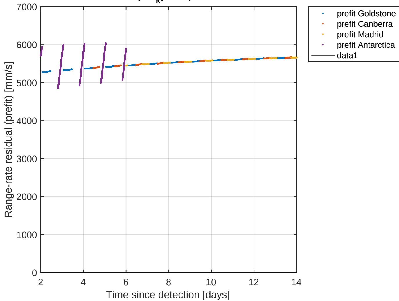
Batch 0to14 (ekf k ): RR prefit residuals
