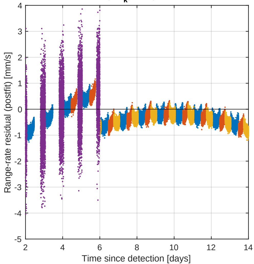
Batch 0to14 (ekf k ): RR postfit residuals
