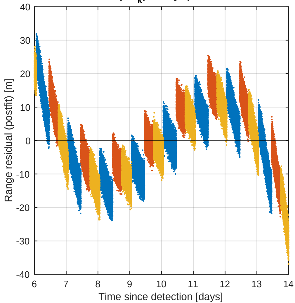
Batch 0to14 (ekf k ): Range postfit residuals
