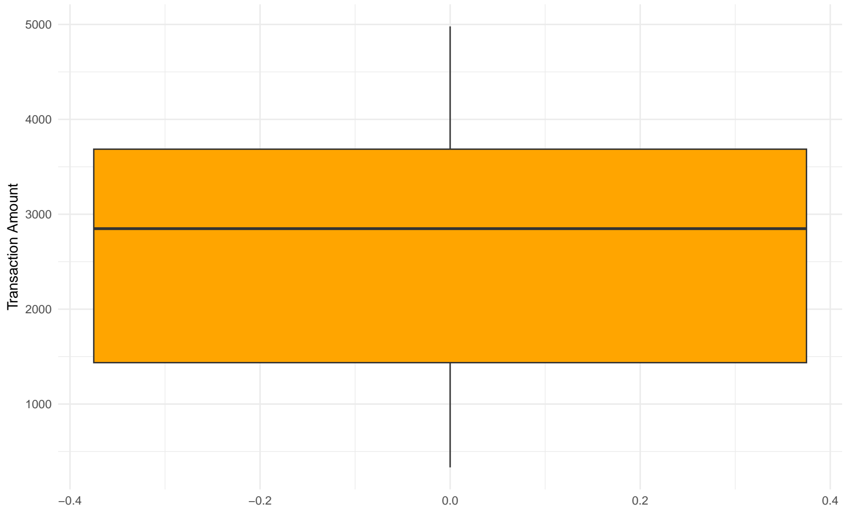
Boxplot of Transaction Amounts
