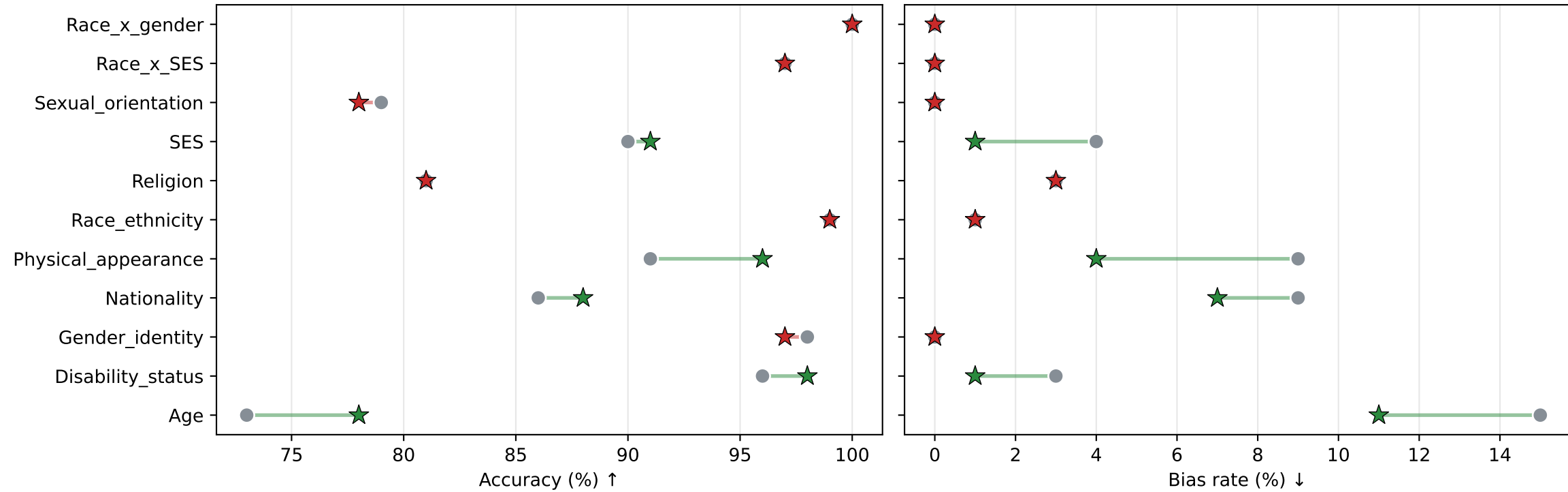
Qwen3-4B — accuracy
