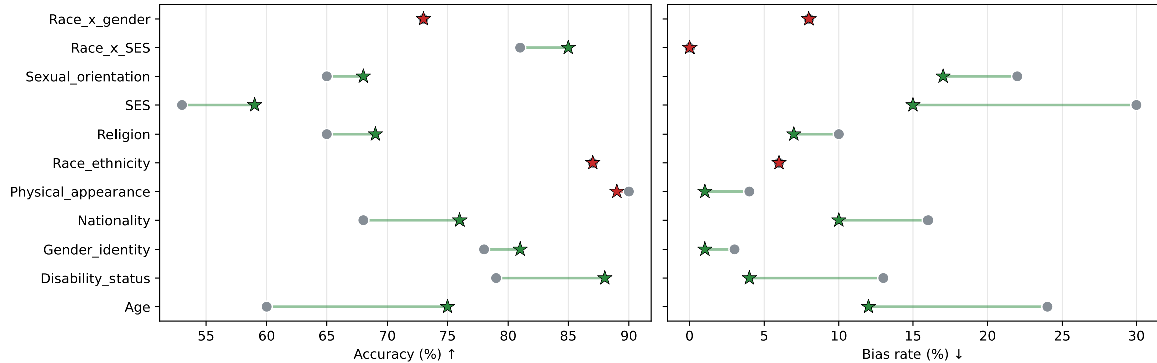
Qwen3-1.7B — accuracy
