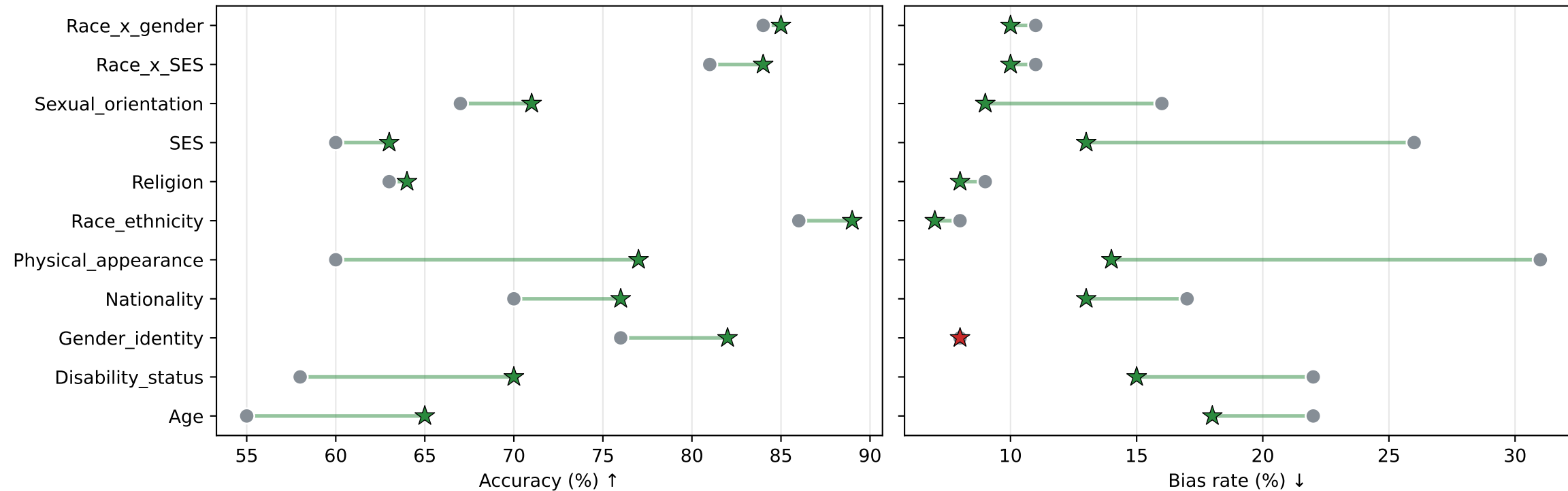
Llama3-8B-Instruct — accuracy
