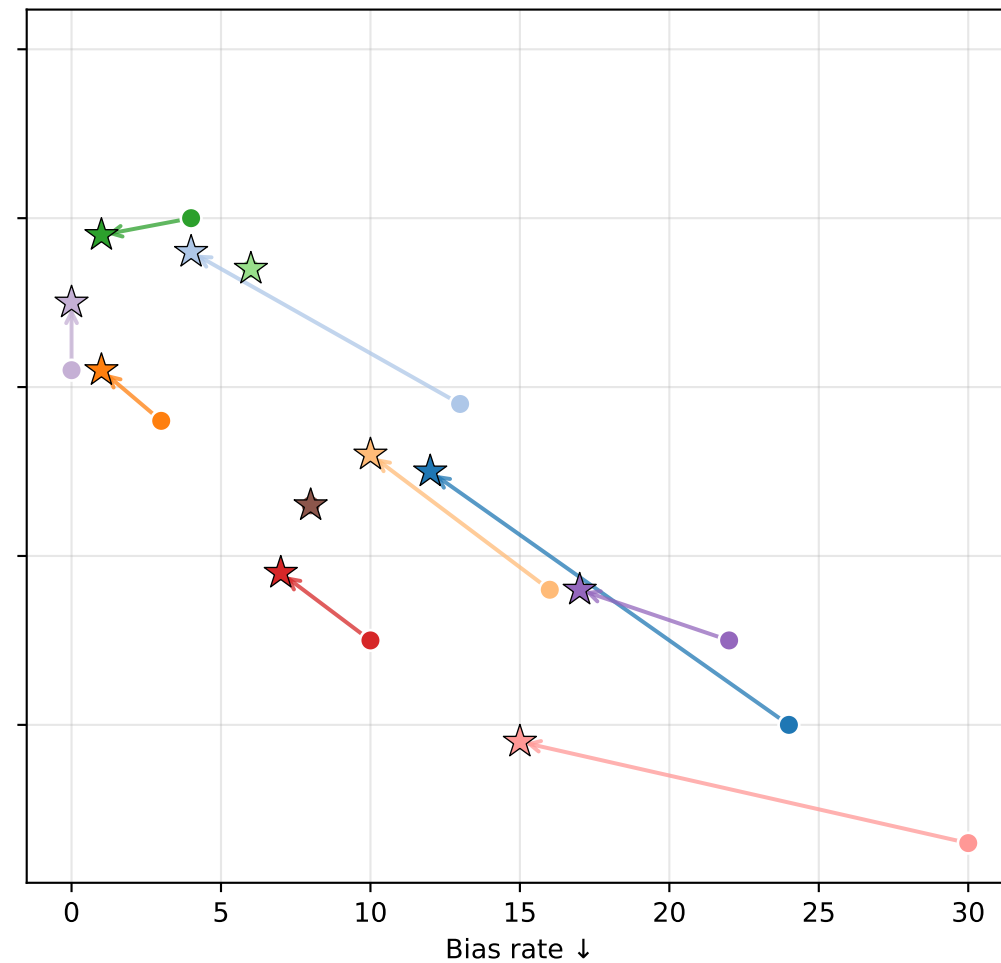
Llama3-8B-Instruct
