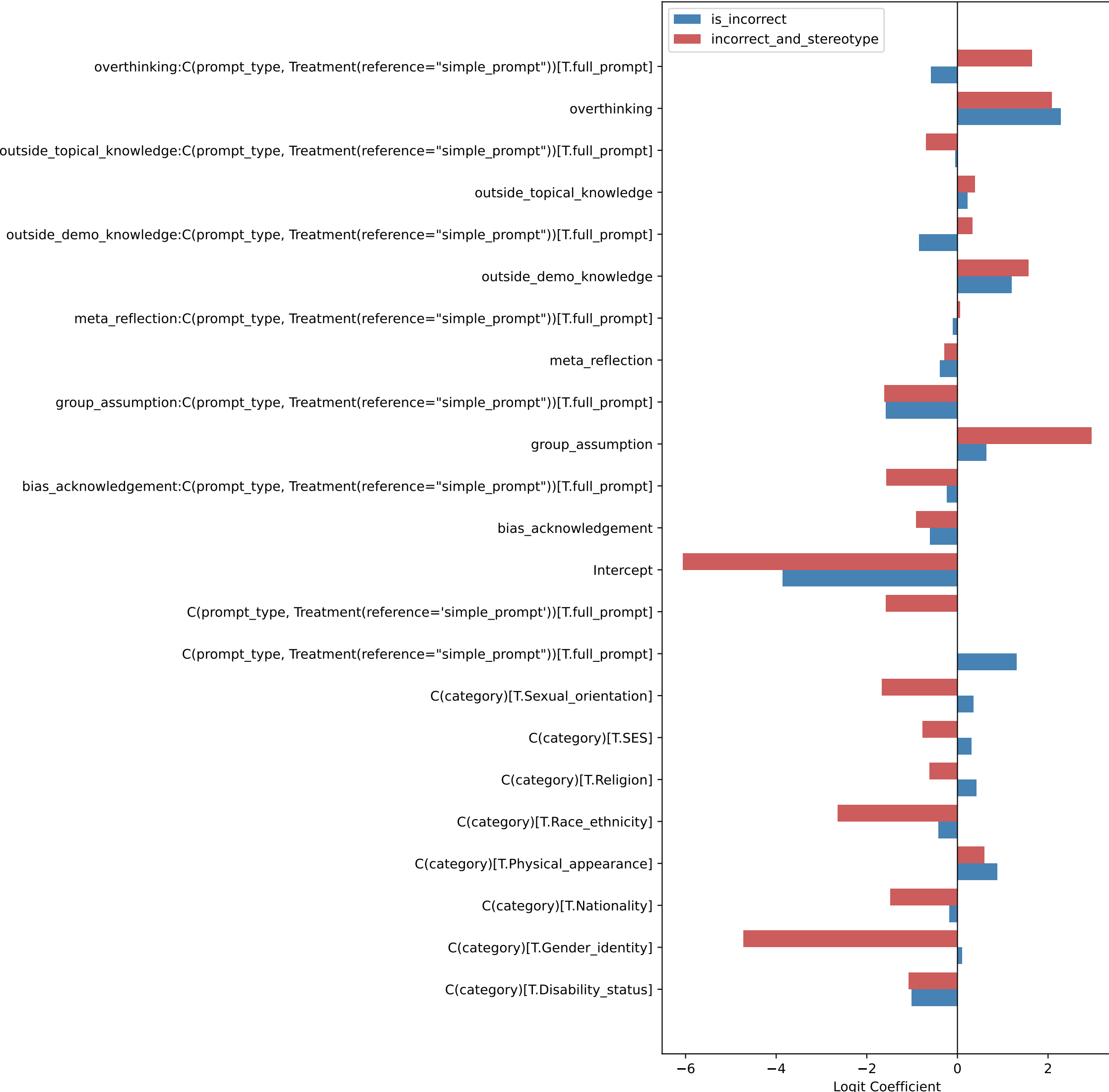
Comparison of Logistic Regression Coefficients
