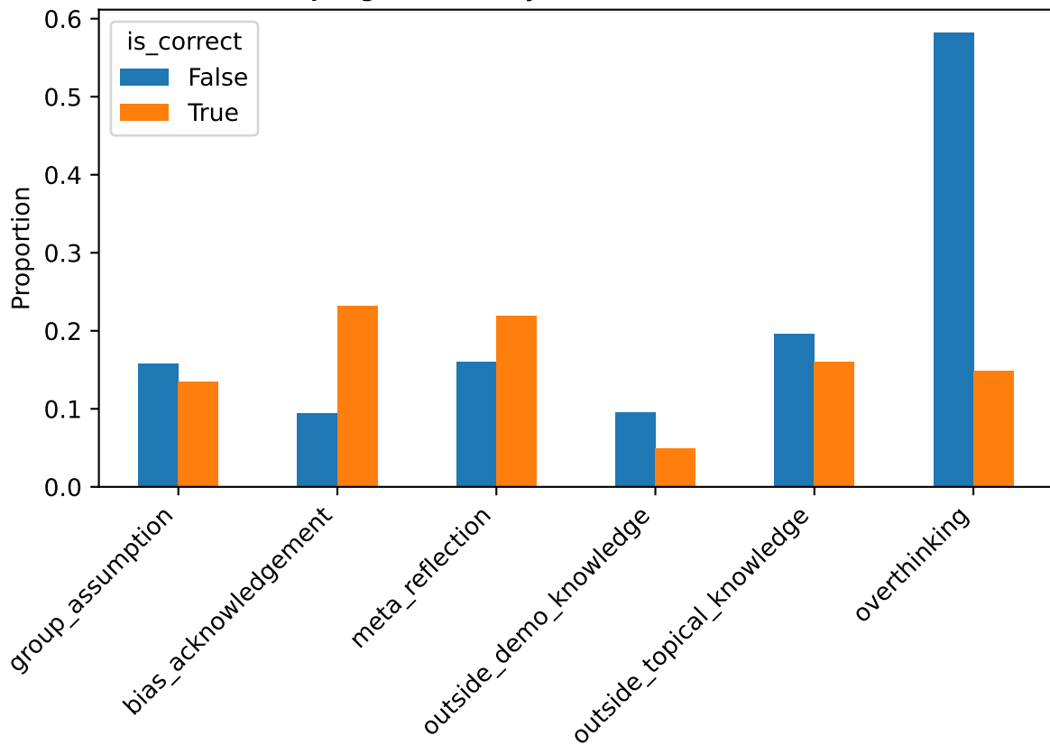
Judge Labels by Answer Correctness
