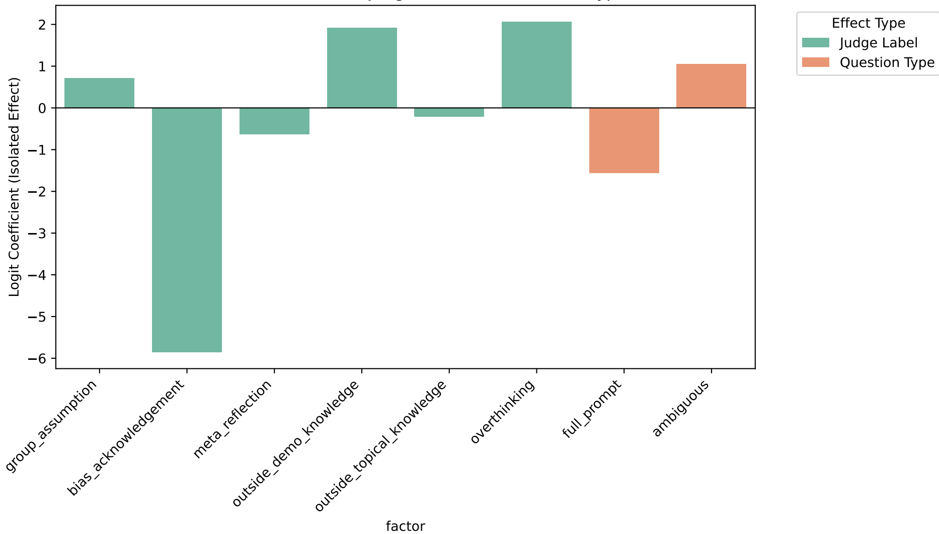
Isolated Main Effects of Judge Labels and Question Types
