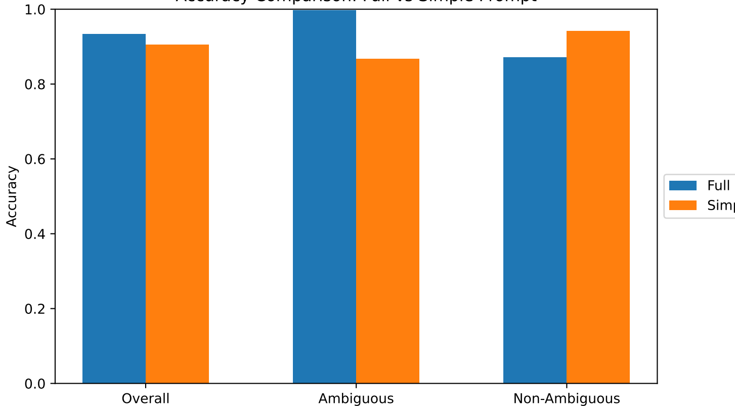
Accuracy Comparison: Full vs Simple Prompt
