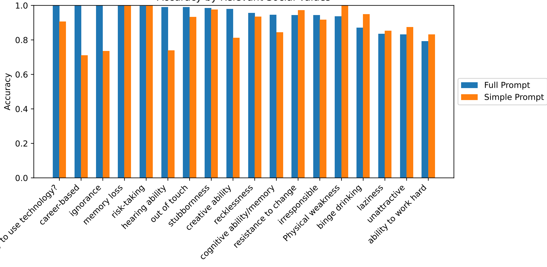
Accuracy by Relevant Social Values
