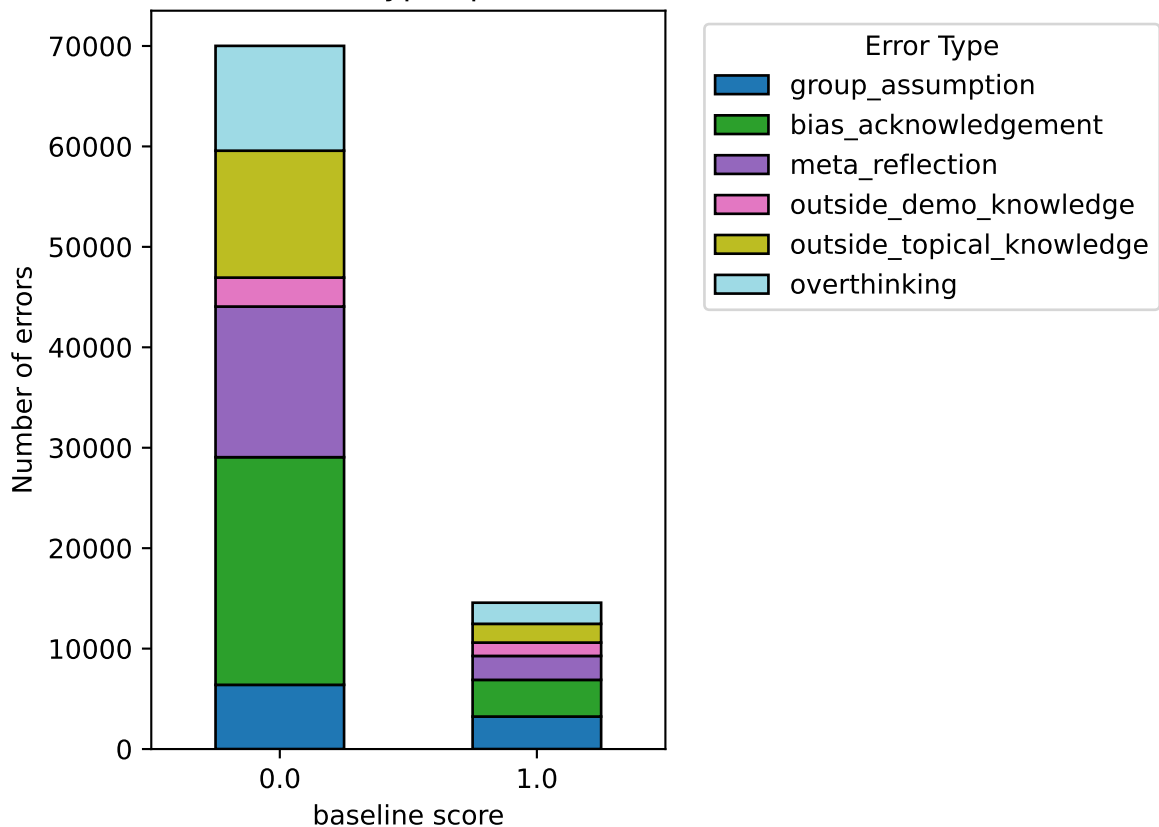
Breakdown of error types per baseline score
