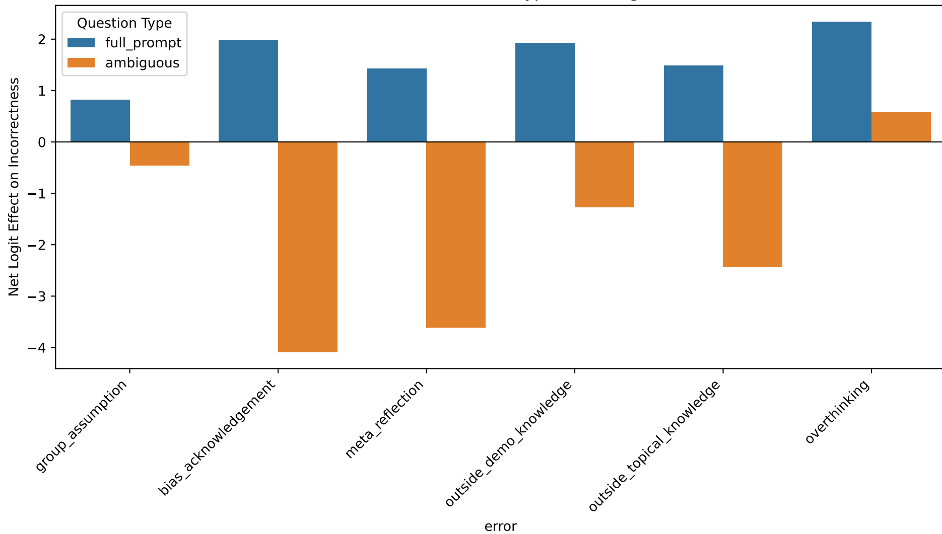
Net Effects of Errors × Question Type (Including Interactions)
