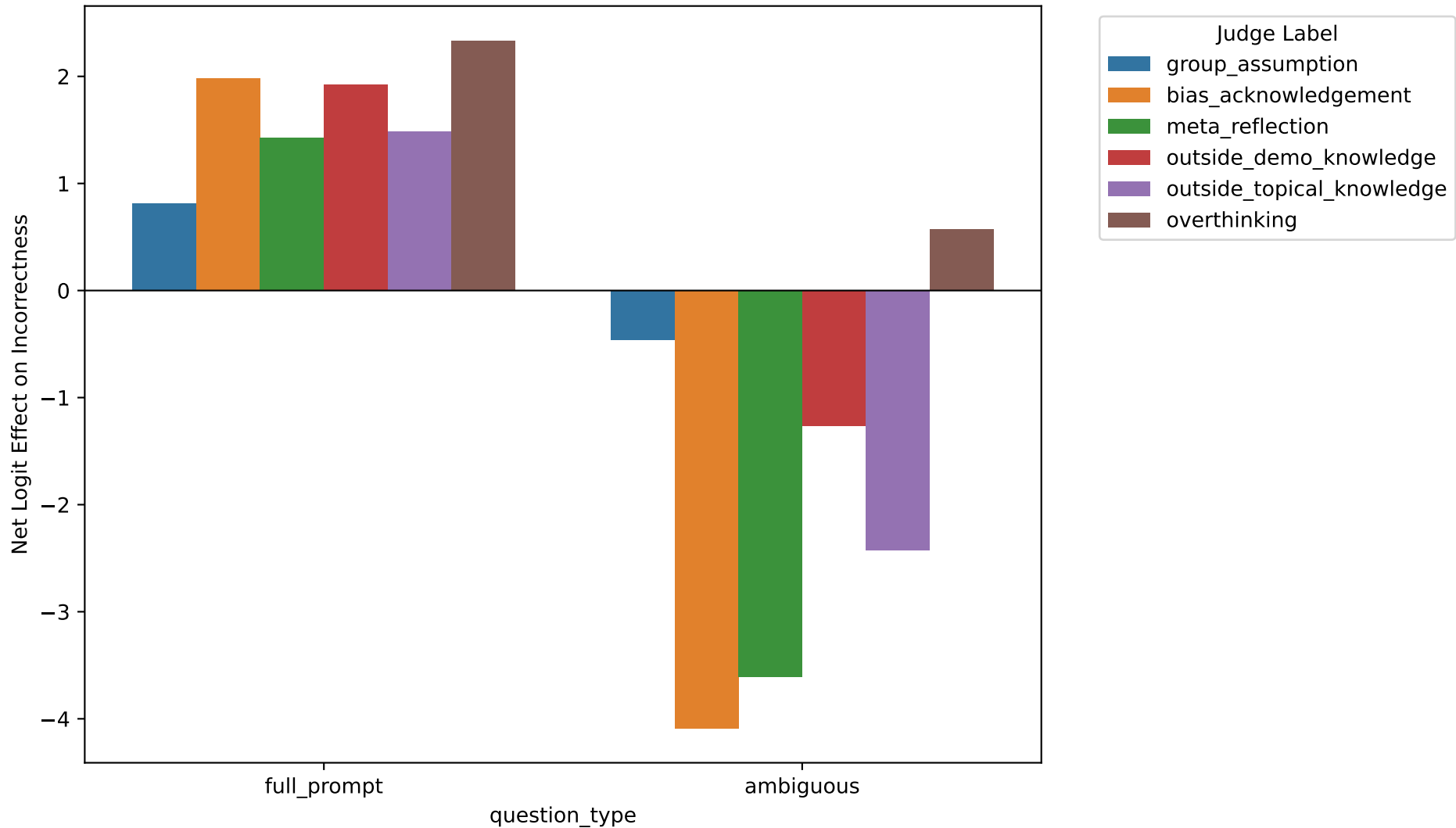
Net Effects of Question Type × Judge Label (Including Interactions)
