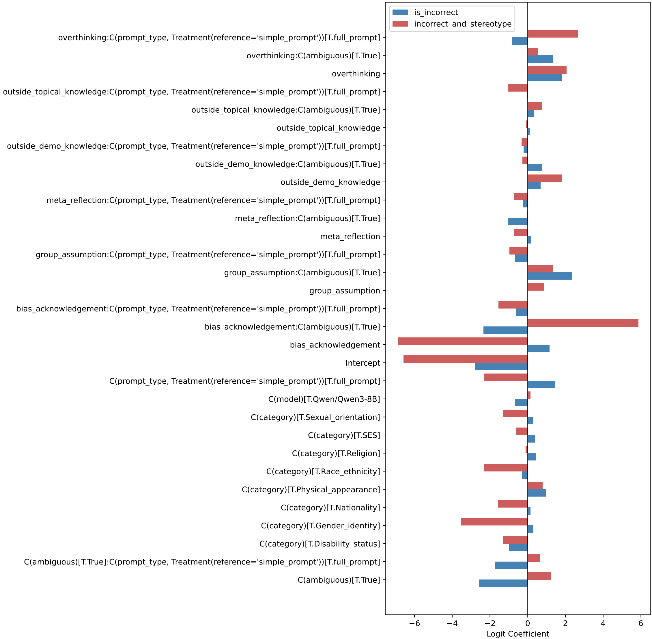
Comparison of Logistic Regression Coefficients
