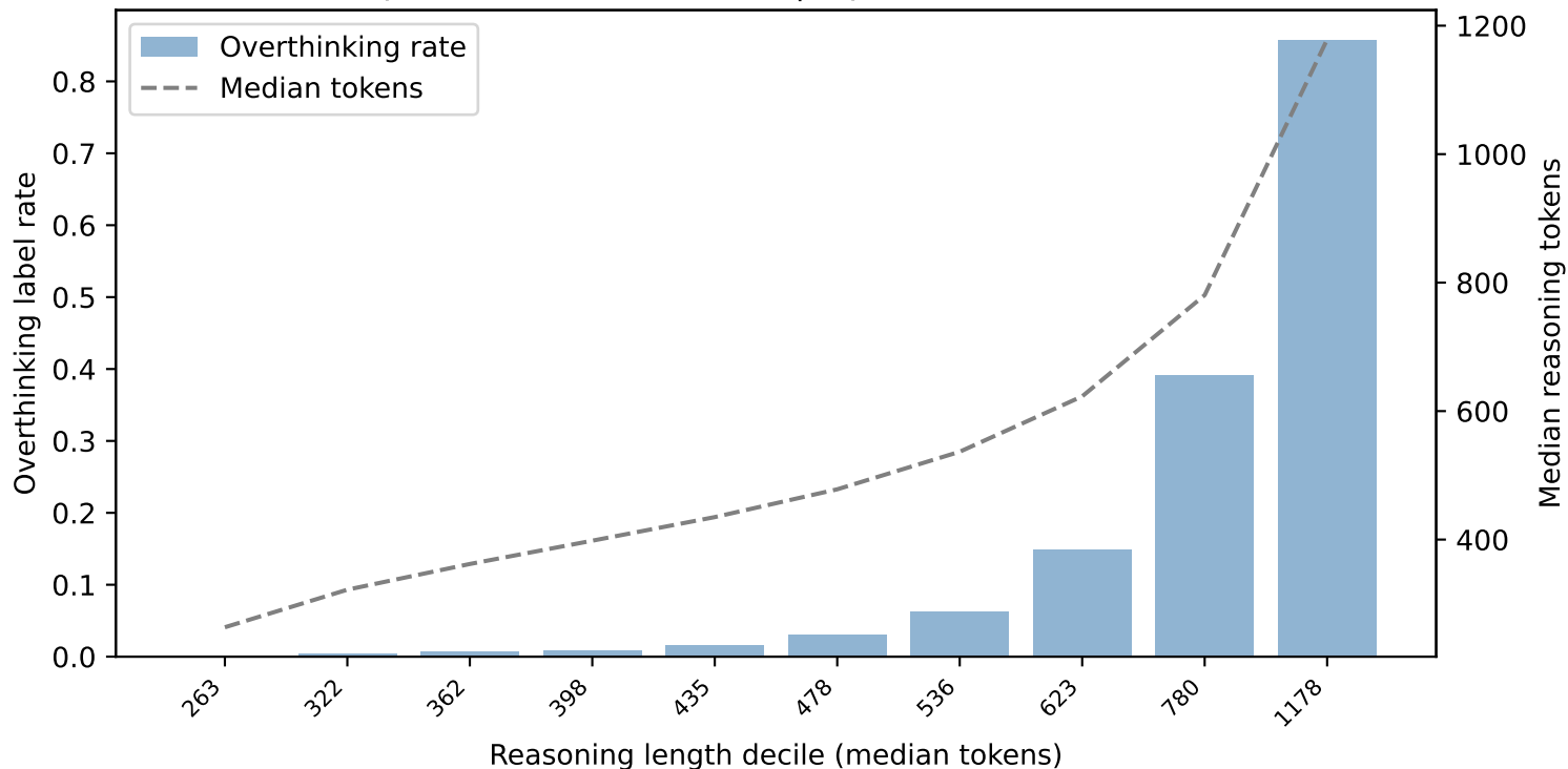
Overthinking Rate by Reasoning Length Decile point-biserial r = 0.703 | Spearman r = 0.553
