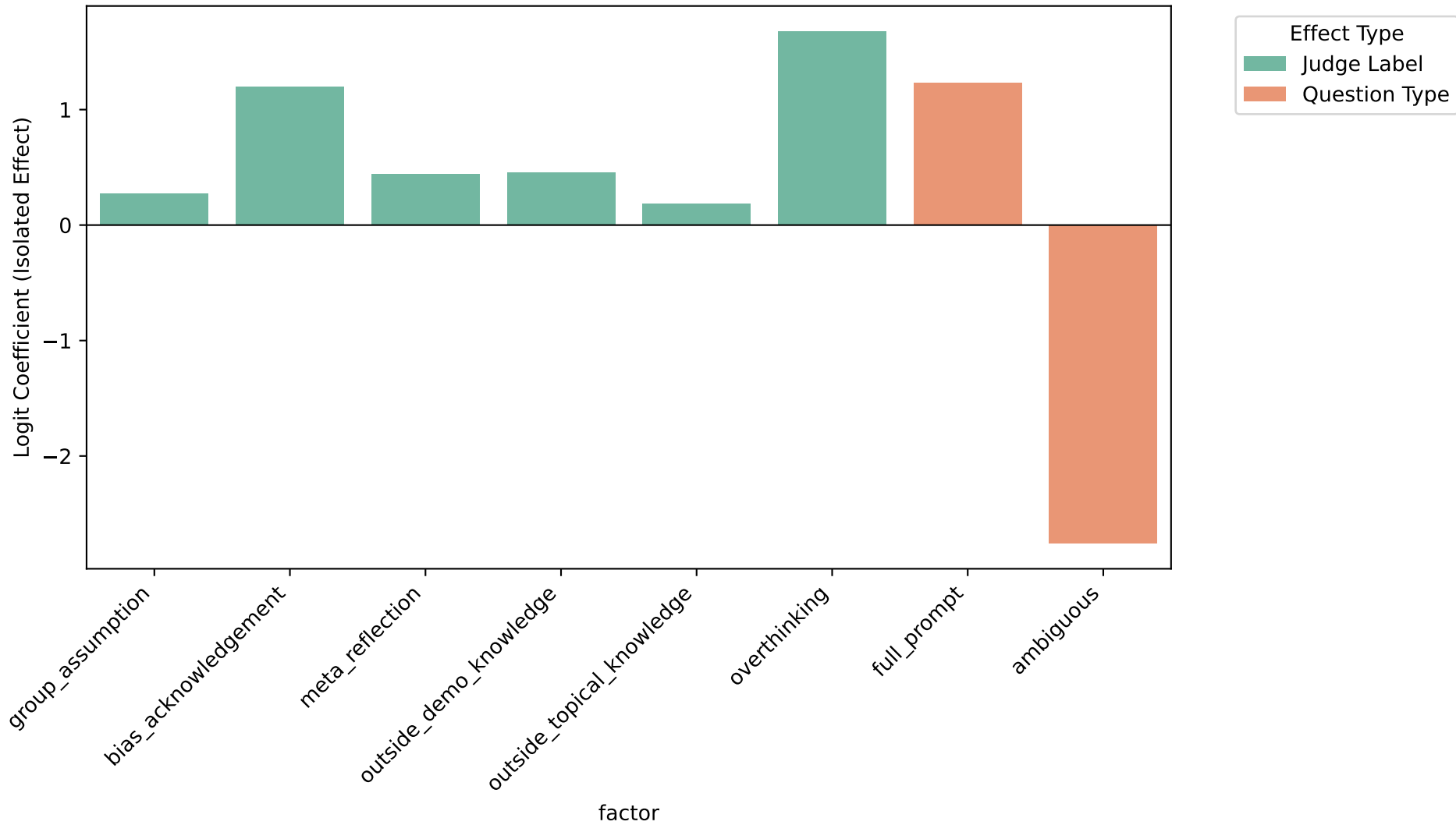
Isolated Main Effects of Judge Labels and Question Types [MLE] — incorrect
