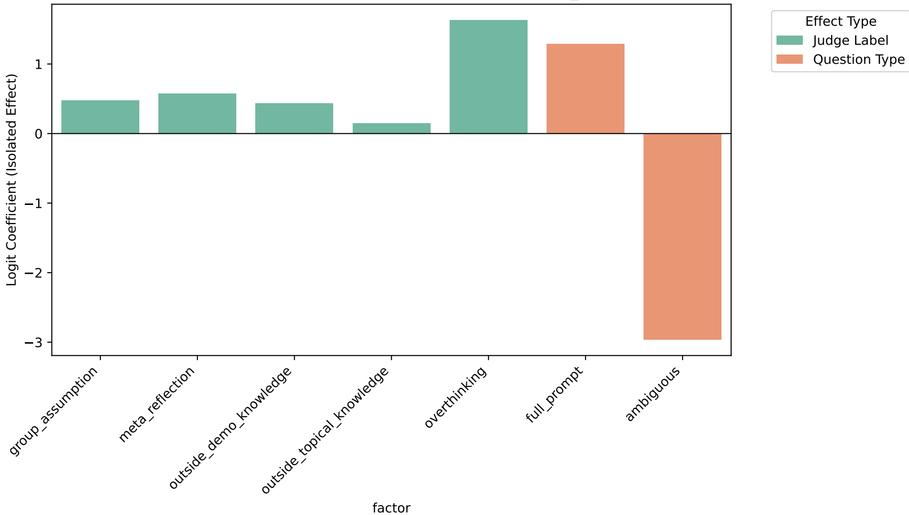
Isolated Main Effects of Judge Labels and Question Types [MLE_nb] — incorrect
