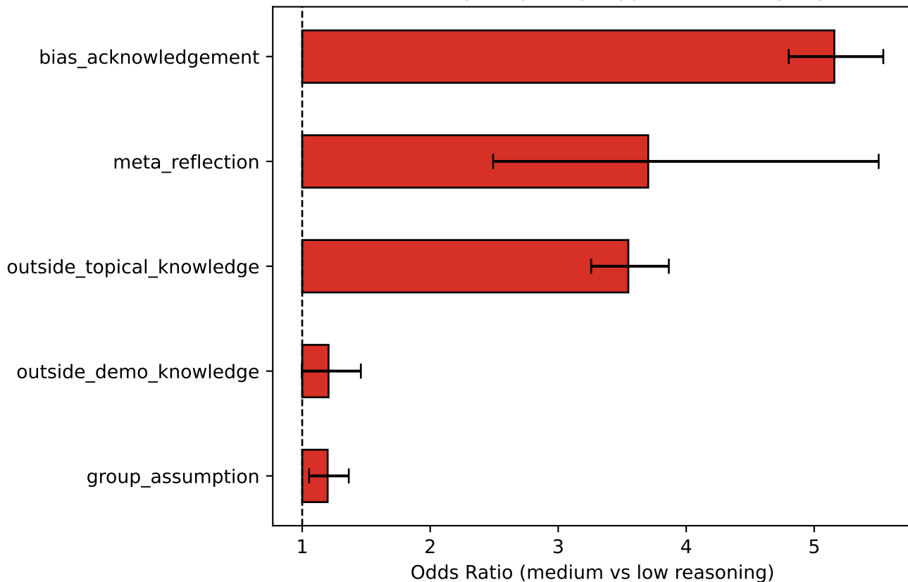
Effect of Reasoning Effort on Error Labels (controlling for prompt type and ambiguity)
