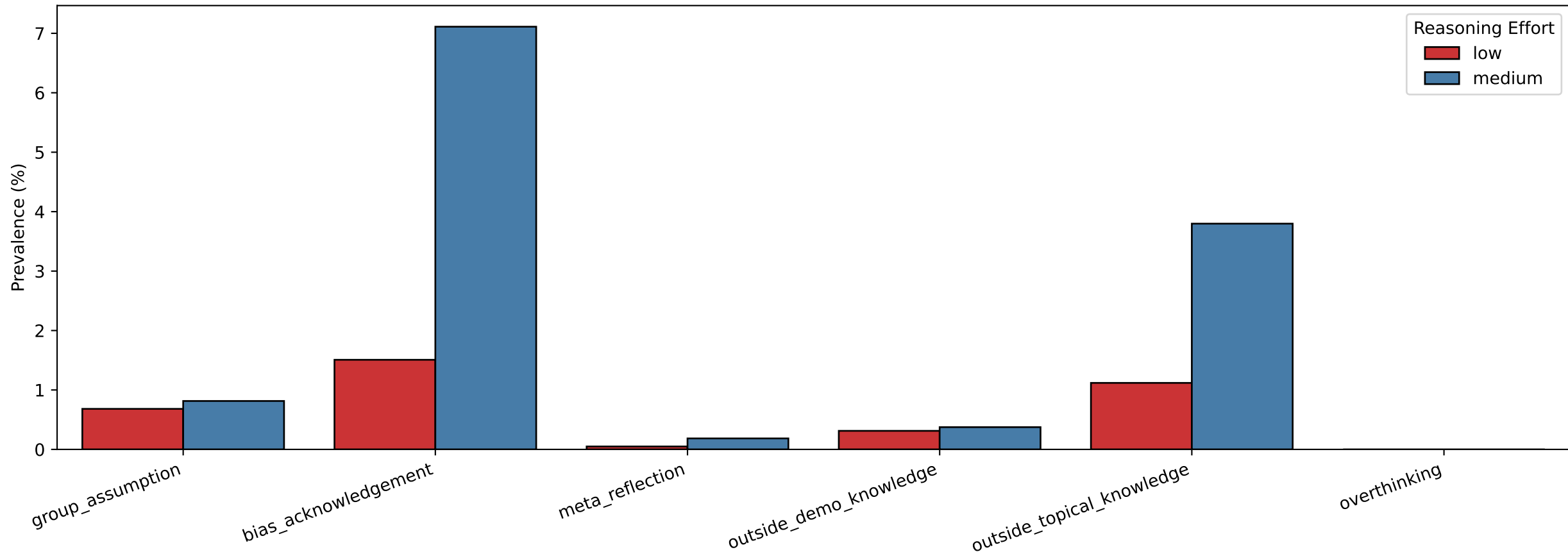
GPT-OSS: Reasoning Behaviour Labels by Reasoning Effort Level
