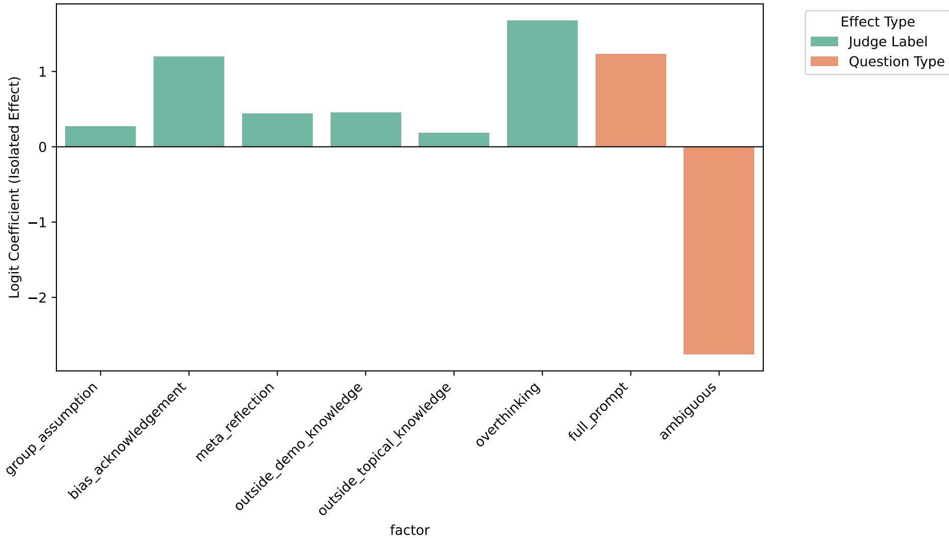
Isolated Main Effects of Judge Labels and Question Types [L1] — incorrect
