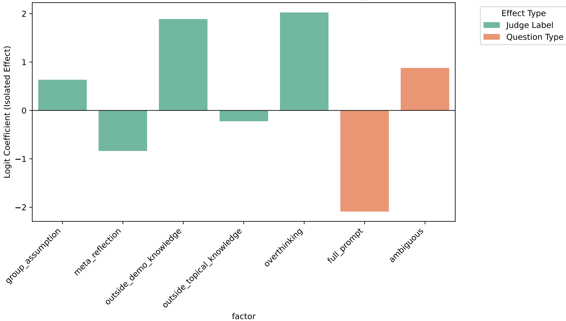
Isolated Main Effects of Judge Labels and Question Types [MLE_nb] — stereo
