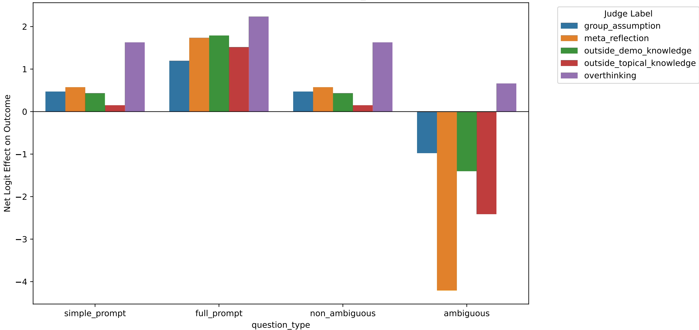
Net Effects of Question Type × Judge Label [MLE_nb] — incorrect
