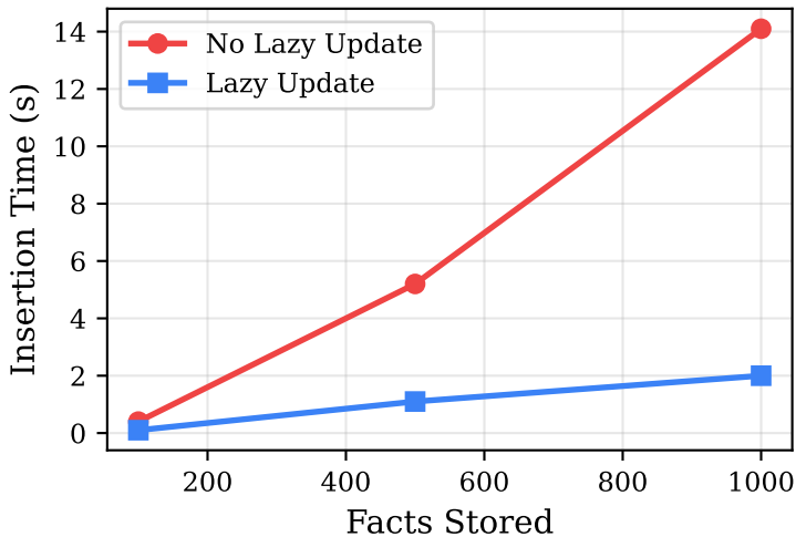
Tree Insertion: Lazy vs No Lazy
