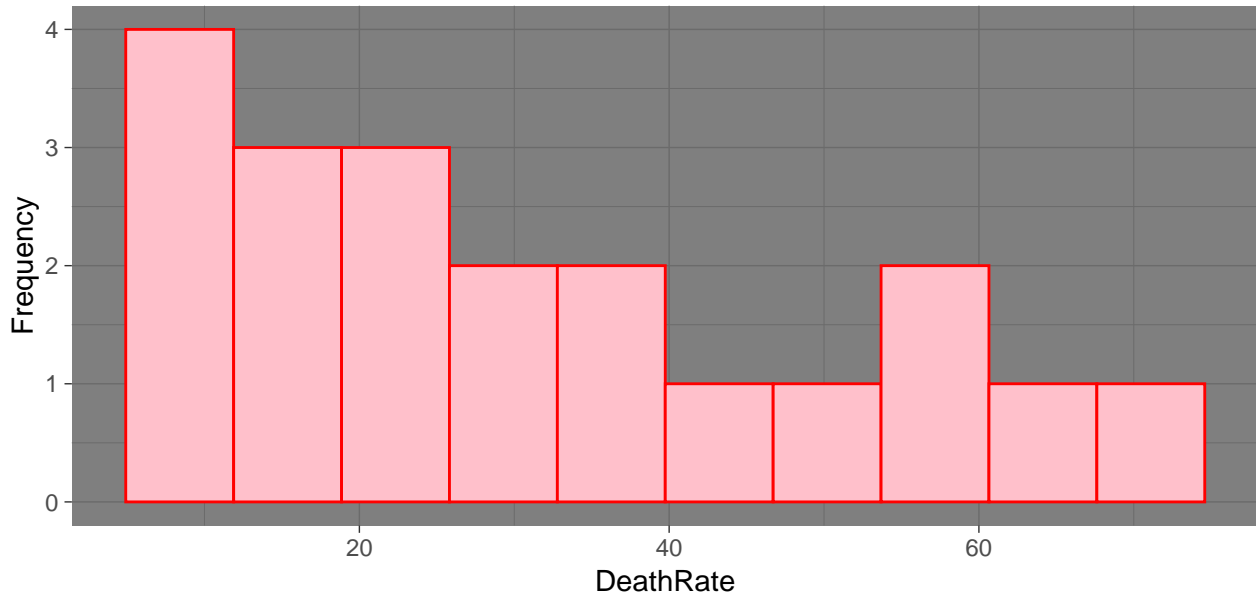
GGPLOT-Histogram
