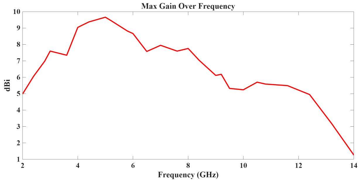
Figure 4: Maximum Gain Over Frequency
