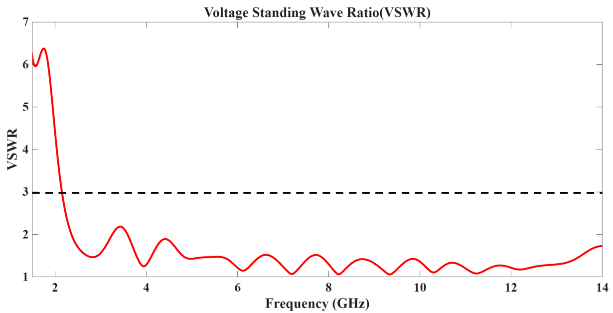
Figure 3: Voltage Standing Wave Ratio(VSWR) plot
