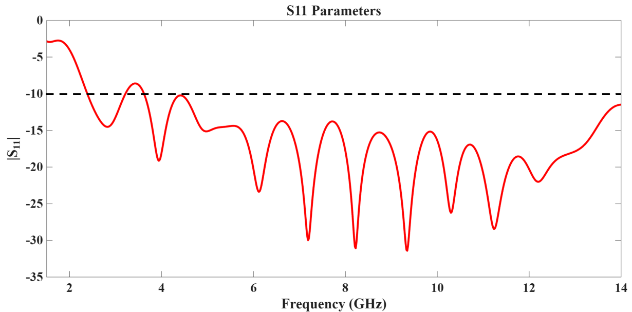
Figure 2: S-Parameters Plot
