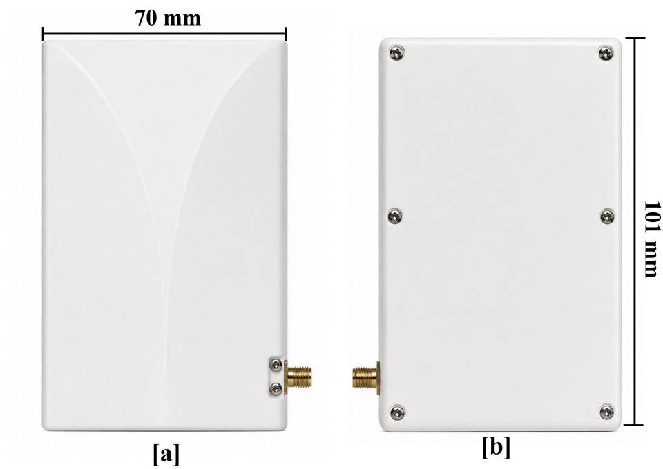
Figure 1: [a] Front View [b] Back View of UWB Vivaldi Antenna
