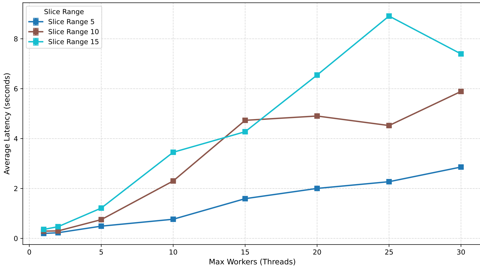
DKRZ: Mean Latency vs Max Workers (All Slice Ranges \pm SEM)
