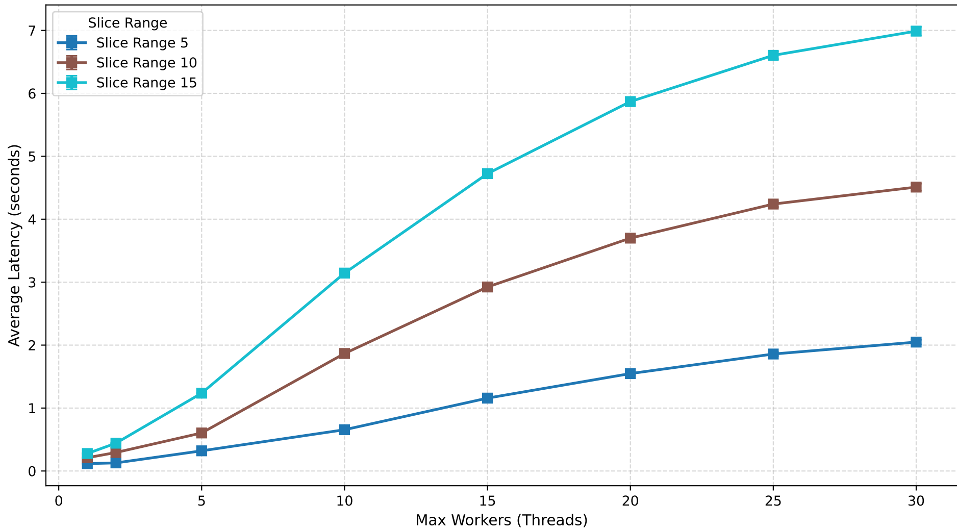
JASMIN: Mean Latency vs Max Workers (All Slice Ranges \pm SEM)
