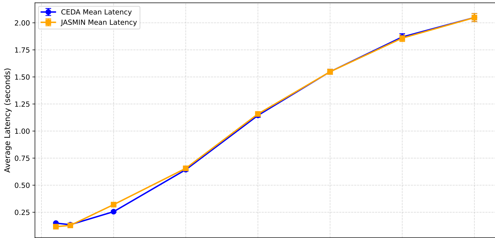
Latency vs Max Workers Comparison (Slice Range = 5 \pm \text{SEM} )
