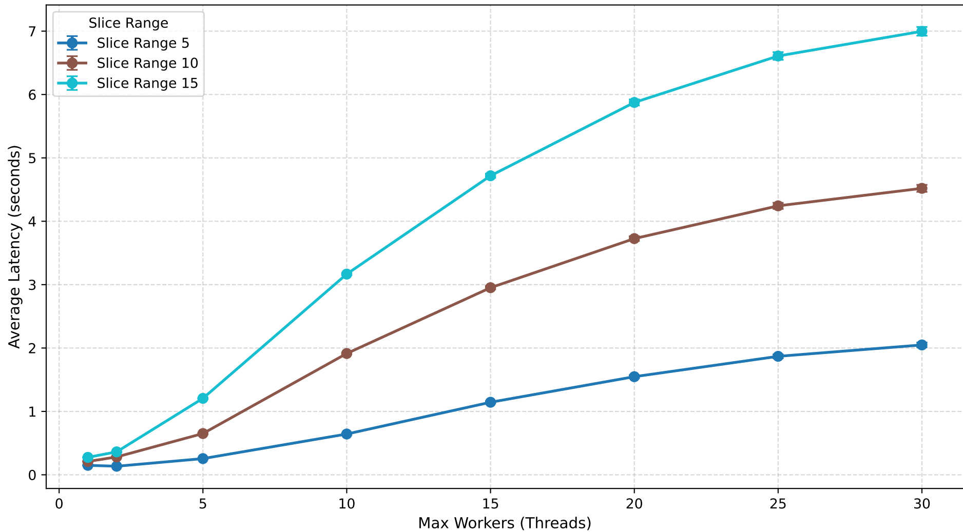
CEDA: Mean Latency vs Max Workers (All Range Slices \pm SEM)
