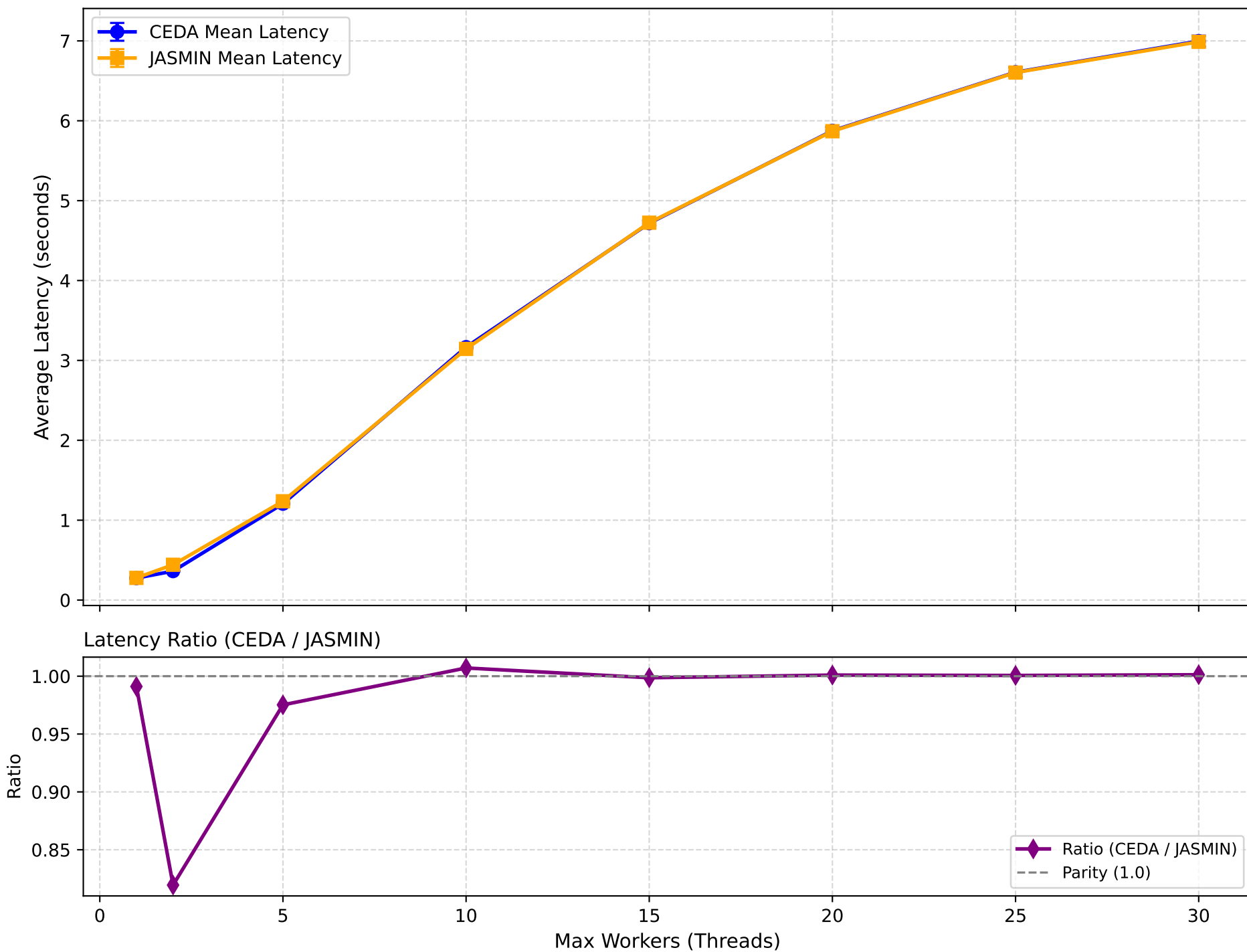
Latency vs Max Workers Comparison (Slice Range = 15 \pm \text{SEM} )
