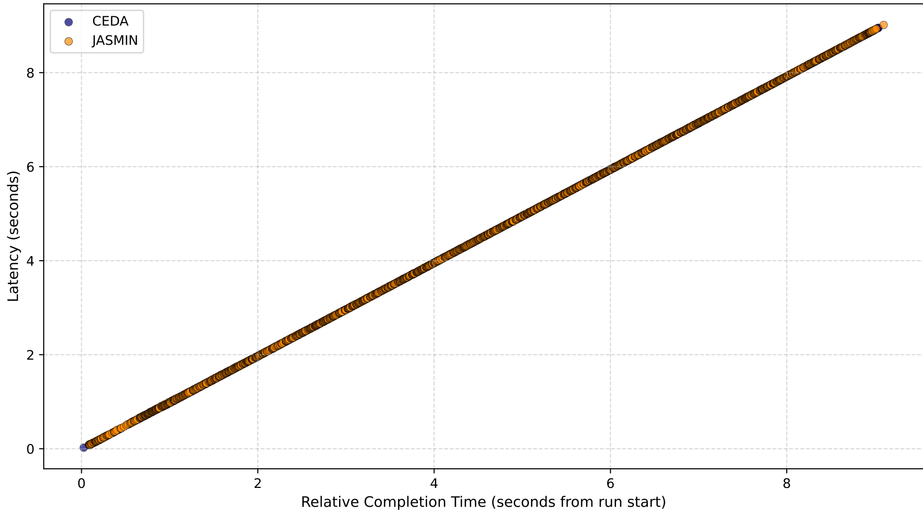
Latency vs Normalized Time | Slice Range: 10 | Max Workers: 30.0
