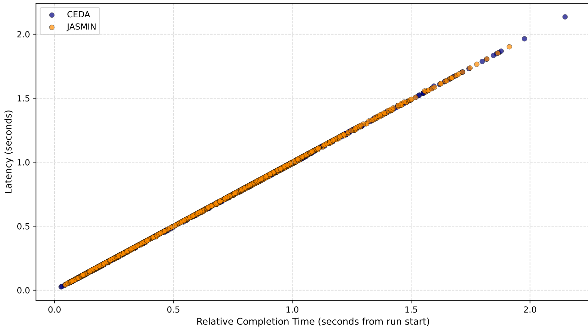
Latency vs Normalized Time | Slice Range: 5 | Max Workers: 10.0
