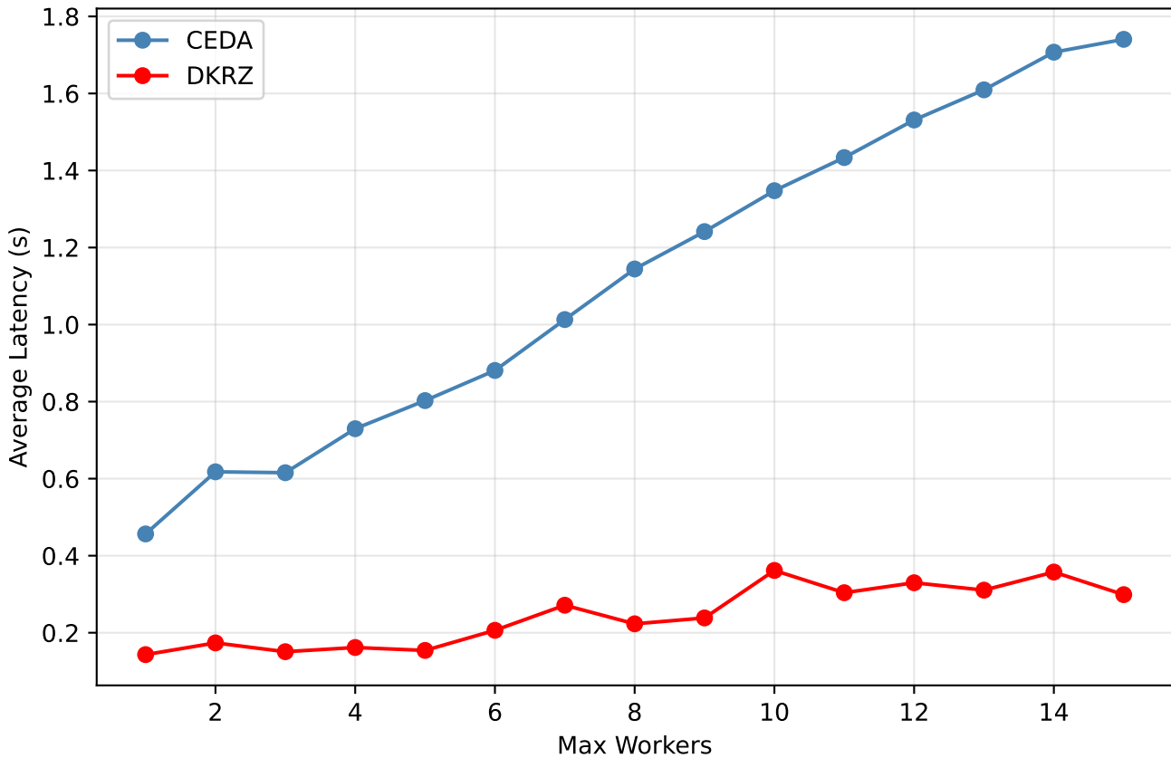
Average Latency vs Max Workers Slice Size=5
