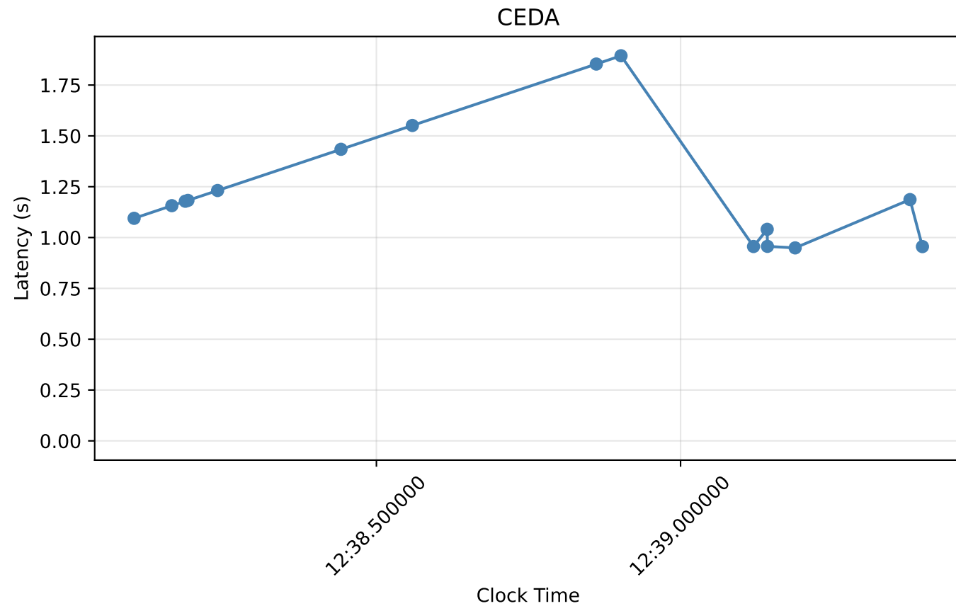
Latency vs Clock Time (Max Workers = 9)
