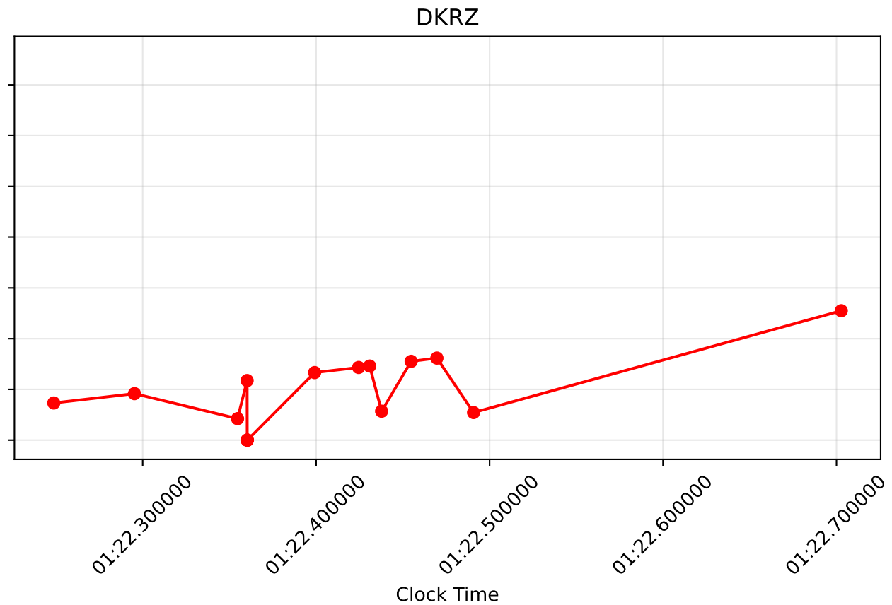
Latency vs Clock Time (Max Workers = 9)
