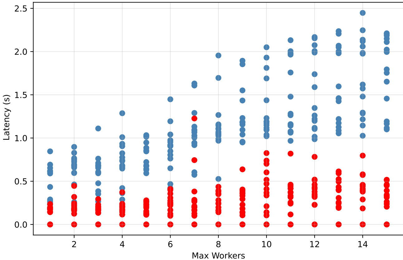
Latency vs Max Workers Slice Size=5
