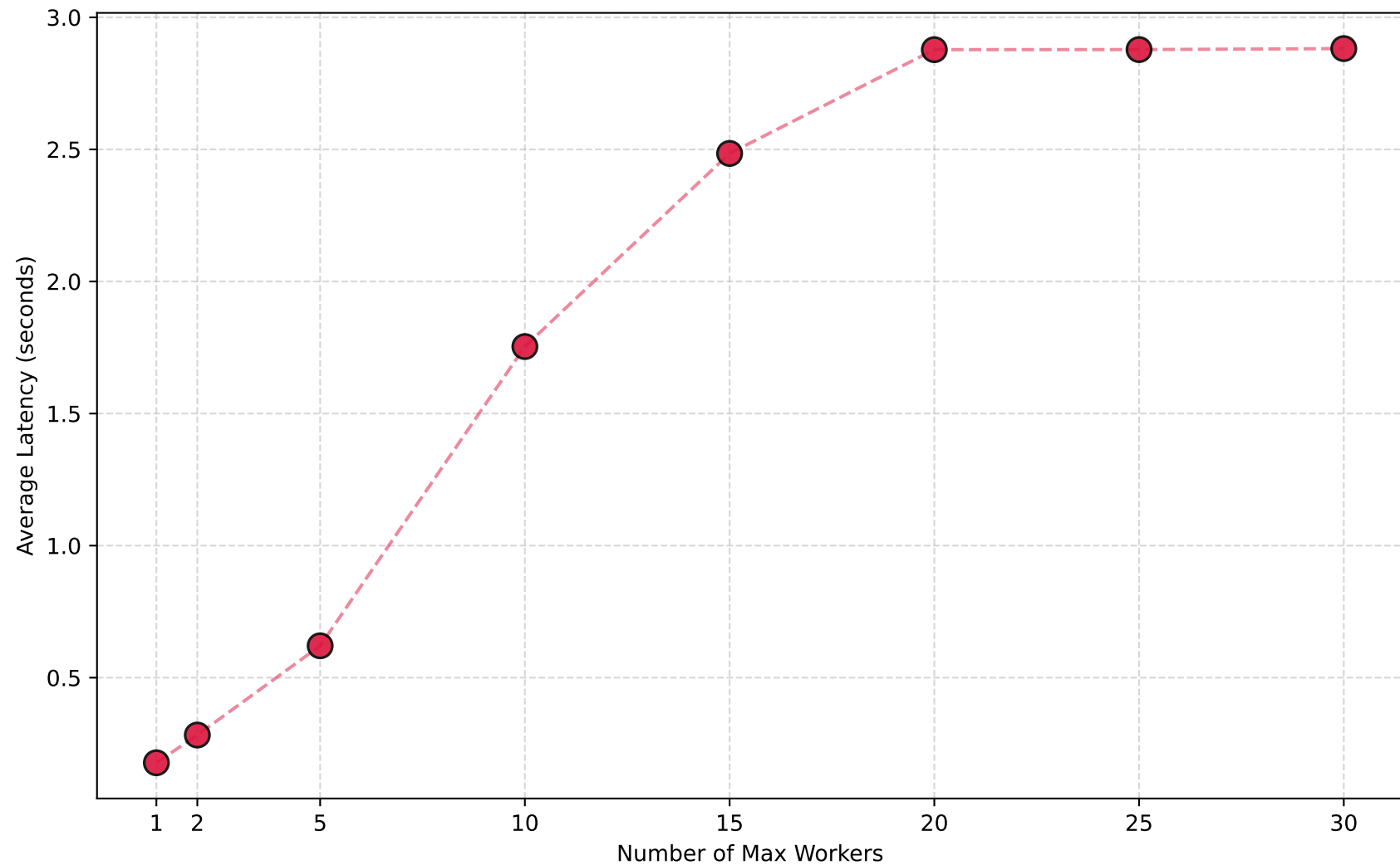
Overall Average Request Latency vs. Max Workers (Chunk Size: 15)
