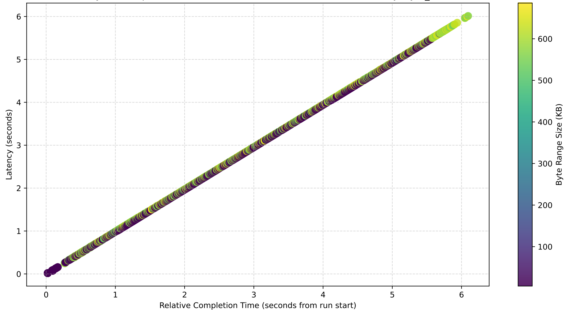
Latency vs. Completion Time (Workers: 20, Chunk Size: 15) (Colored by: byte_size)
