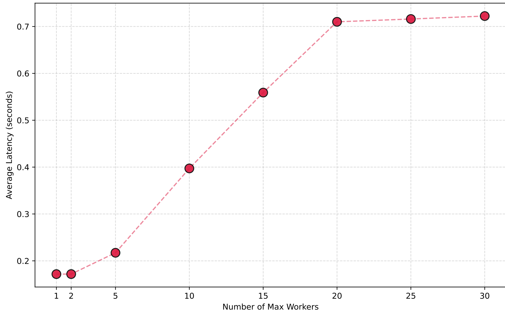
Overall Average Request Latency vs. Max Workers
