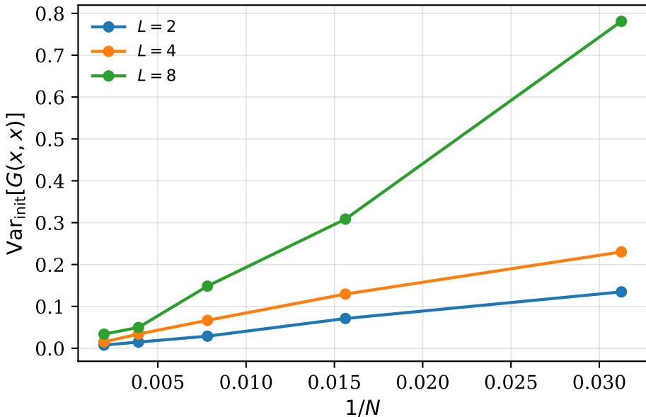
deep linear metric fluctuations \sim L/N
